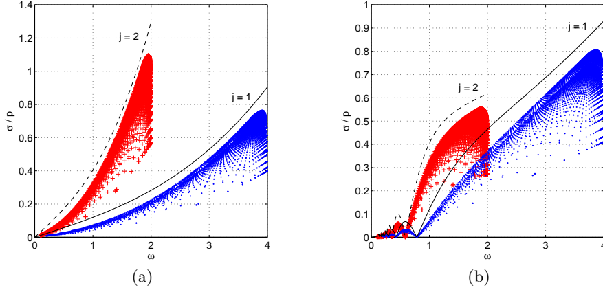
FIGURE 6. Rescaled inviscid growth rates \sigma/p at resonance as a function of \omega , for different values of j = 1, 2 as marked in the figure and comparison with maximum local instability growth rate (eq. 3.16 with C = -1/2 ) (full and dashed lines). We consider triangular deformation n = 3 in a cylinder with height h = 2 . In (a) we fix the libration angle \Delta\varphi = 1 , in (b) we fix the libration amplitude \varepsilon = 1 . The survey involves all modes up to n_{r,max} = 2 , m_{1,max} = 50 , n_{z,max} = 50 .
