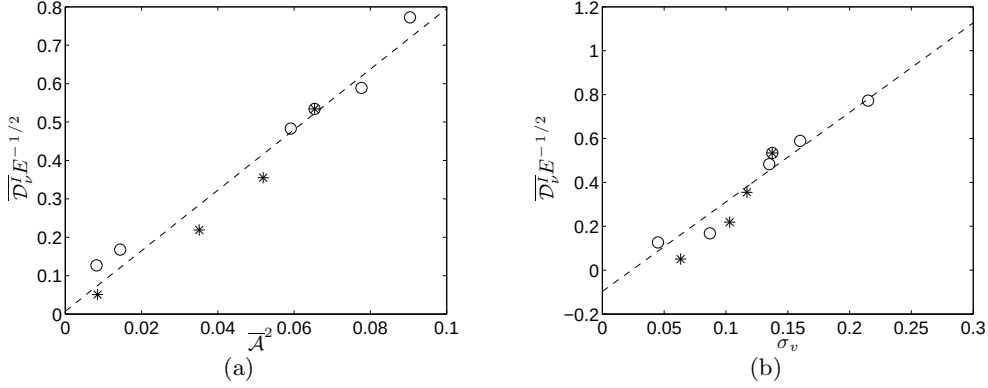
FIGURE 17. Evolution of the viscously rescaled dissipation E^{-1/2}\overline{\mathcal{D}}_\nu^I for n = 3 , \omega = 3 , \varepsilon = 1 , p = 0.45 and E = 1.5 \cdot 10^{-3}, 10^{-3}, 7 \cdot 10^{-4}, 5 \cdot 10^{-4}, 2.5 \cdot 10^{-4}, 10^{-4} (o) and p = 0.3, 0.37, 0.4, 0.45 , E = 5 \cdot 10^{-4} (*), dashed lines being linear fits of the data points. (a) In function of \overline{\mathcal{A}}^2 , i.e. the square of the amplitude of the equilibrated flow driven by the LDMI. (b) In function of the growth rate \sigma_v .
