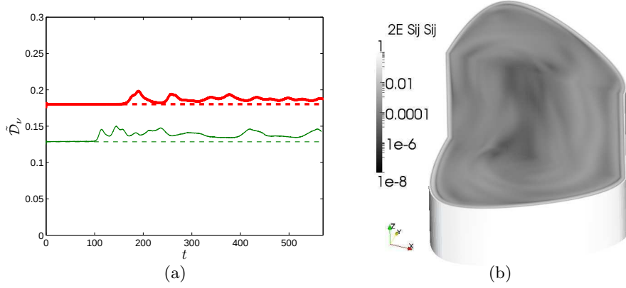
FIGURE 16. (a) Moving average \tilde{\mathcal{D}}_\nu of the viscous dissipation of the flow for n = 3, \omega = 3, \varepsilon = 1, p = 0.4, E = 5 \cdot 10^{-4} (thick) and p = 0.45, E = 2.5 \cdot 10^{-4} (thin). Dashed lines indicated the average dissipation \mathcal{D}_\nu^L of the laminar base state. (b) Snapshot of the local viscous dissipation rate 2ES_{ij}S_{ij} for n = 3, \omega = 3, \varepsilon = 1, p = 0.4, E = 5 \cdot 10^{-4} at t = 424 .
