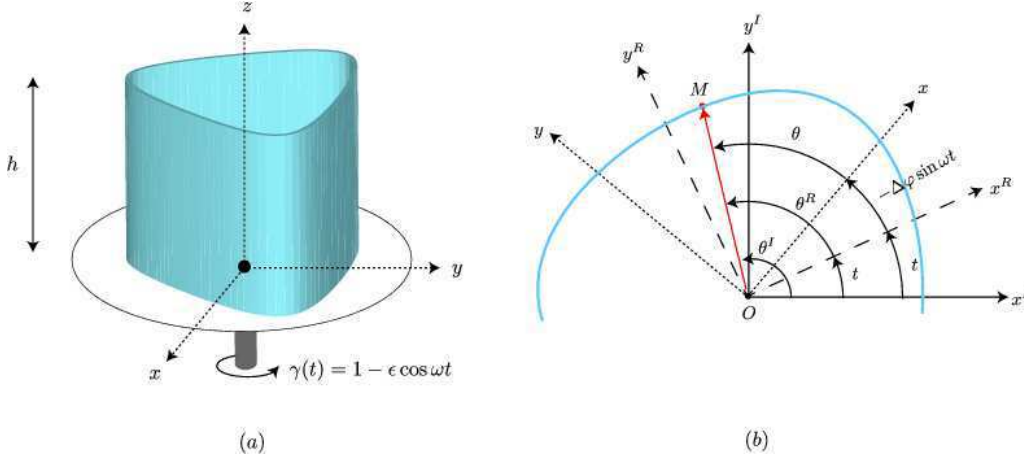
FIGURE 1. (a) Sketch of the studied set-up. A deformed cylinder is put on a turntable that rotates at the dimensionless rotation speed \gamma(t) = 1 - \varepsilon \cos \omega t . The combination of libration and deformation drives a 2D basic flow, which can be destabilized into 3D flows through the Libration Driven Multipolar Instability (LDMI). (b) Different frames of reference are used: the librating frame (x, y, \theta) , no superscript) attached to the turntable, the inertial (or lab) frame (x^I, y^I, \theta^I) and the frame rotating at constant speed 1 (x^R, y^R, \theta^R) .
