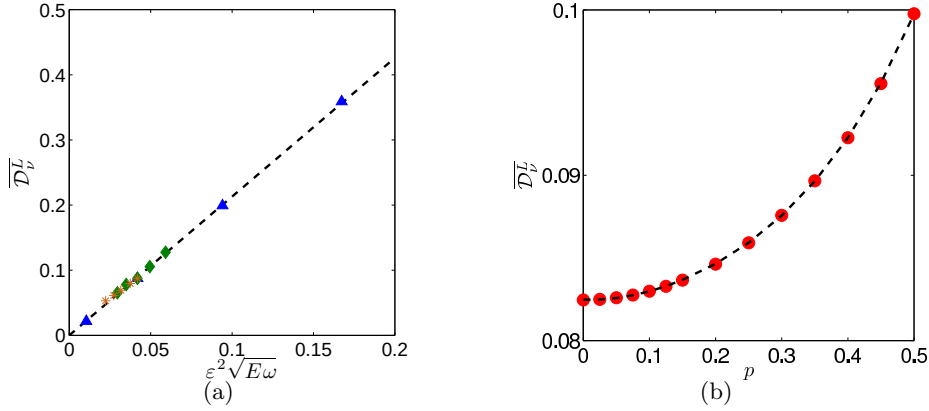
FIGURE 19. Viscous dissipation rate \overline{\mathcal{D}}_\nu^L of the two-dimensional basic flow for n = 3 . (a) in function of \varepsilon , E and \omega with fixed p = 0.3 . Triangles: varying \varepsilon , fixed E = 5 \cdot 10^{-4} and \omega = 3.5 , diamonds: varying E for fixed \varepsilon = 1 and \omega = 3.5 , asterisks: varying \omega for fixed \varepsilon = 1 and E = 5 \cdot 10^{-4} . Dashed line: linear fit to the data points, giving a slope of 2.13. (b) in function of p for fixed E = 5 \cdot 10^{-4} , \varepsilon = 1 and \omega = 3.5 . Circles: numerical data points, dashed line: fourth-order polynomial fit to the data points.
