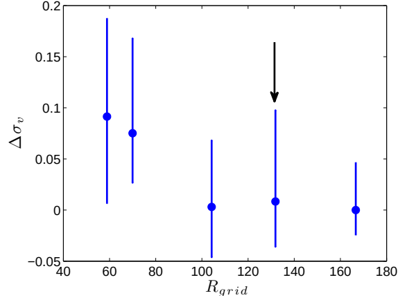
FIGURE 9. Convergence of the growth rate of a 3D multipolar instability with increasing grid resolution (for E = 5 \cdot 10^{-4} , n = 3 , p = 0.45 , \varepsilon = 1 , \omega = 3 ). For each simulation at a given mesh resolution R_{grid} , we perform several measures of \sigma , which gives several measures of the relative difference \Delta\sigma_v . We report in this figure the mean value of \Delta\sigma_v (dots), as well as the obtained extremum values (errorbars). The arrow indicates the minimal resolution used for the systematic study of the instability in subsection 4.3.
