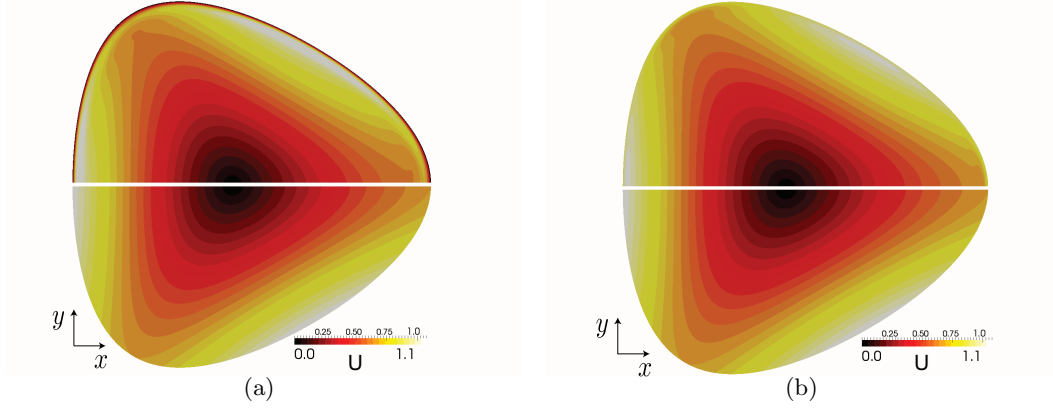
FIGURE 11. Comparison for n = 3 , p = 0.3 , E = 5 \cdot 10^{-4} , \omega = 2.5 and \varepsilon = 1 between the exact basic flow (2.8) (bottom half) and the numerically established 2D basic flow (top half) for the case of a rigid tripolar ( n = 3 ) container (a), and a deformable container, deformed by rollers (b).
