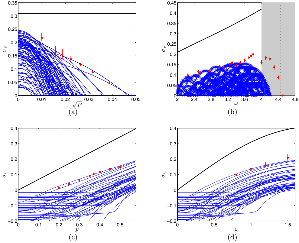
FIGURE 13. Growth rate \sigma_v in function of the flow parameters E , p , \varepsilon and \omega for n = 3 . Results of the asymptotic WKB analysis (thick black line) given by (3.16) for C = -1/2 (boundary pathline), global analysis (thin blue lines and blue crosses) and numerical simulations (red circles). (a) In function of E for \varepsilon = 1 , p = 0.45 , and \omega = 3 , (b) in function \omega for \varepsilon = 1 , p = 0.45 and E = 5 \cdot 10^{-4} , (c) in function of p for \omega = 3 , \varepsilon = 1 and E = 5 \cdot 10^{-4} , and (d) in function of \varepsilon for \omega = 3 , p = 0.45 and E = 5 \cdot 10^{-4} .
