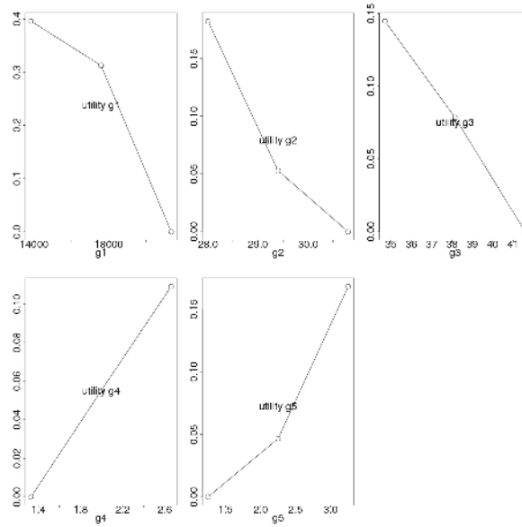
Figure 4: Plots of the partial value functions
