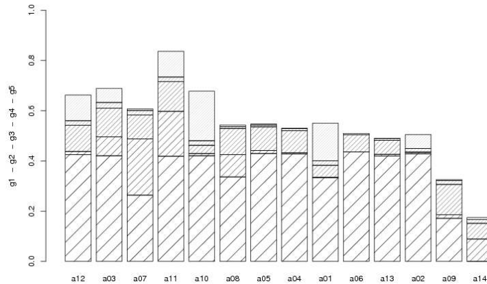
Figure 3: Graphical representation of the normalized performance table.
