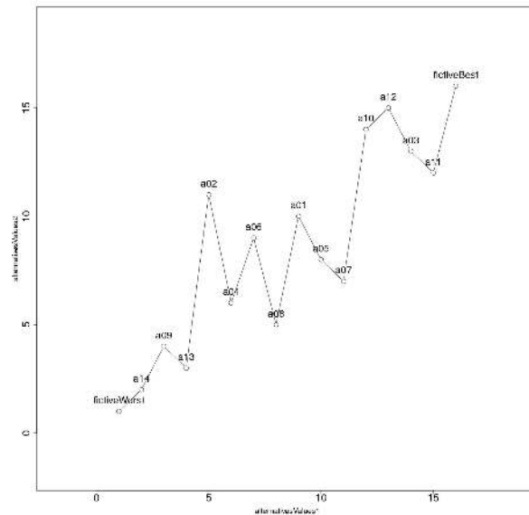
Figure 5: XY plot representing both rankings (abscissa: ranks by ACUTA, ordinate: ranks by the weighted sum)
