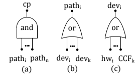
Fig. 2. Device failure condition.
