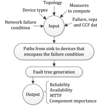
Fig. 1. Overview of the methodology for common cause failure analysis.
