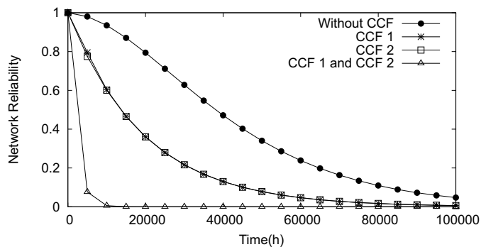
Fig. 4. Network reliability analysis considering common cause failure.
