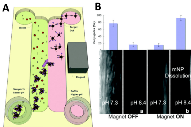
Fig.13 Target analyte separation, in a microfluidic channel, facilitated by pH-responsive magnetic nanoparticles (MNPs). The left stream (green) is the sample that has been pre-incubated with MNPs. MNP aggregation is induced by using a lower pH buffer in this sample flow stream. The pH of the right stream (pink) is chosen to reverse MNP aggregation. A rare-earth magnet provides sufficient magnetic field to attract the aggregates laterally into the higher pH flow stream, where they return to a dispersed state, carrying the bound target analyte with them (A). Fluorescence microscopy results showing continuous stream purification of streptavidin-MNP conjugates. When the magnetic field is applied, the conjugate aggregates moved laterally across to the higher pH flow stream, where they redisperse. When the magnetic field is applied, most conjugates were moved into the high pH stream and 80% of the conjugates were collected from the right outlet (B). Adapted from ref. 38 with permission of The Royal Society of Chemistry.
