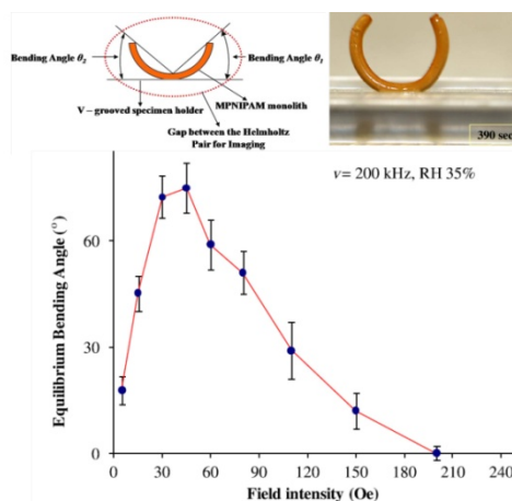
Fig. 4 Magnetic PNIPAM ferrogel cylinder lying on a grooved substrate undergoing bending under RF magnetic field due to the strain difference between the contact area with the solid under tension and the free surface under compression due to gel de-swelling when temperature reaches the LCST of PNIPAM by magnetic induction (adapted from ref. 13 with permission from the IOP Publishing).
