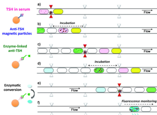
Fig.14 Diagram illustrating the basic steps involved in the magnetic immunoassay. Using an initial trap ( ie. magnetic tips, opposed triangles on the scheme), antibody-grafted magnetic nanoparticles contained in the first drop were captured and transferred to a second sample drop composed of thyroid-stimulating hormone (TSH) in serum (a, b). After incubation in the capillary loop following the first tweezers, the magnetic nanoparticles with the antibody complexes were trapped again in the same tweezers and washed with a droplet of buffer to remove non-specifically adsorbed proteins (c). The beads were resuspended and incubated in a fourth droplet containing the enzyme-labelled secondary antibody (d). Washing was performed in the second magnetic trap with three successive buffer droplets (e) to remove unbound secondary antibodies. Finally, the particles were released and incubated with a fluorogenic enzymatic substrate and the output was read (f). Adapted from ref. 39 with permission from John Wiley and Sons, copyright 2012.
