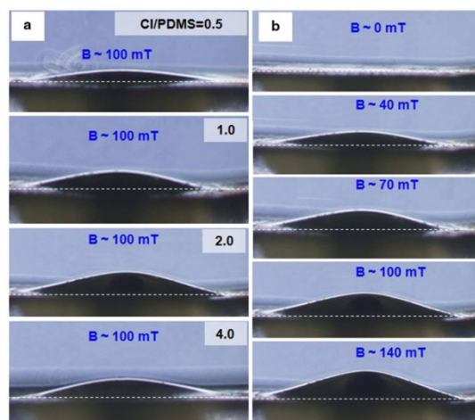
Fig. 6 a) Deflection of different membranes ( \sim 1.0 mm in diameter, 100 \mu\text{m} in thickness) under the same magnetic field ( H = 80 kA/m, B = 100 mT) at increasing weight ratios CI/PDMS from 0.5 to 4; b) Deflection of the same membrane (weight ratio = 2) for increasing fields up to H = 112 kA/m. Such membranes can be used to design pumps or valves in a microchip (Reprinted from ref. 16 with kind permission from Springer Science and Business Media).
