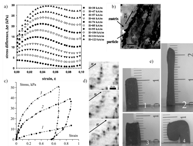
Fig. 5 Behaviours of MR/MA elastomers in homogenous magnetic fields; a–c) MR silicone loaded at 25 vol% with soft iron pre-aligned under a field H = 123 kA/m during the curing step; a) plot illustrating the influence of increase of magnetic field intensity H on the traction curve expressed as the difference of stress \Delta\sigma for a given strain \epsilon relatively to the curve without applied field H = 0 ; b) optical micrograph showing chains of magnetic fillers; 14 ; c–e) unstructured MA elastomer at 30–35 vol% of magnetic phase in a uniform magnetic field; c) Stress-strain dependence at (1) H = 0 , (2) H = 96 kA/m, and (3) H = 208 kA/m showing a residual strain under magnetic field; d) under an increasing applied magnetic field H , the embedded CI fillers form chains, before returning to their initial positions when the field is switched off; e) picture of the initial shape (1) and of the deformed shapes retained after stretching (2), contraction (3) or bending (4) as long as the magnetic field is maintained; relaxation occurs when the field is switched off (Adapted from ref. 14 and 15 with permission from the World Scientific Publishing Co and IOP Publishing, respectively).
