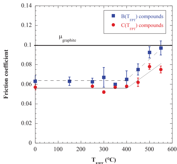
Figure 1 Evolution of friction coefficient (recorded after three cycles) as a function of fluorination post-treatment temperature for B(T_{FPT}) and C(T_{FPT}) materials
