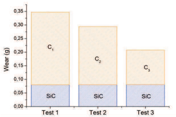
Figure 3 Wear loss.
