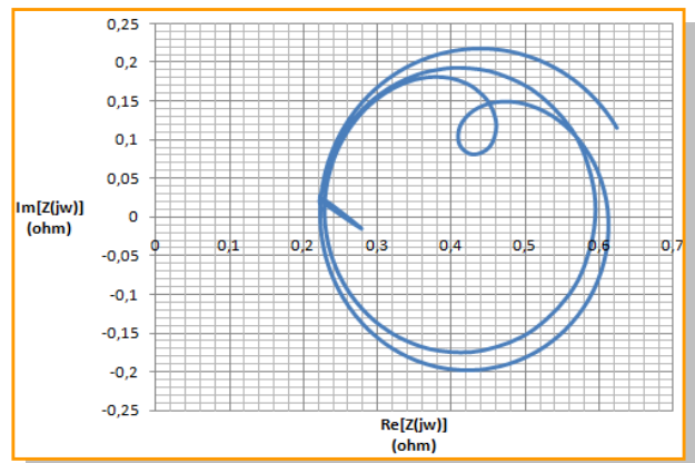
Fig. 8. Nyquist diagram of a healthy DFIG.
