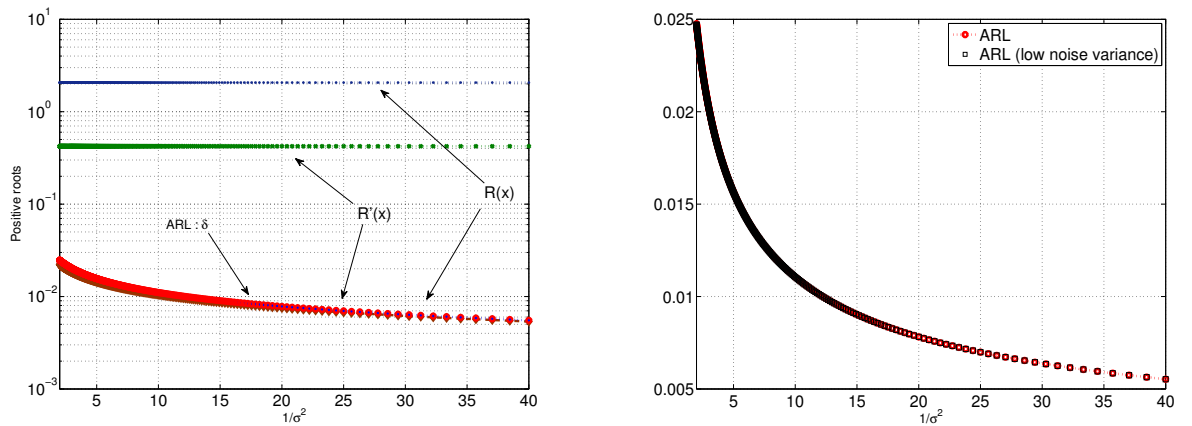
Figure 1. (a) Positive roots for polynomials R(x) , R'(x) and analytic ARL given in expression (24) vs. the inverse of the noise variance. (b) ARL given in expression (24) and the approximated ARL under the assumption of low noise variance given in expression (26) vs. the inverse of the noise variance.
