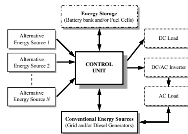
Fig. 2. Hybrid generation systems general architecture.
