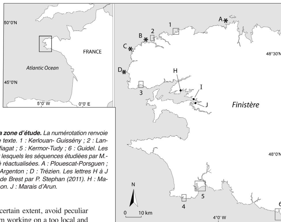
Fig. 1 – Location maps of the study area. Numbers refer to sites presented in the text. 1: Kerlouan-Guissény; 2: Landeda-Tariec; 3: Porsmilin; 4: Treffiagat; 5: Kermor-Tudy; 6: Guidel. Letters A to D refer to sites from which sedimentary sequences were re-assessed from M.-T. Morzadec-Kerfourn (1974). A: Plouescat-Porsguen. B: Ploudalmezeau-Treompan. C: Argenton. D: Trézien. Letters H to J refer to sites studied by P. Stephan (2011) in the Bay of Brest. H: Porzguen marsh. I: Troaon marsh. J: Arun marsh.
