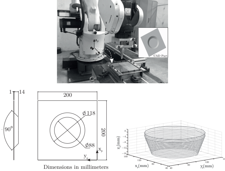
Figure 10: Experimental setup and target tool path of the frustum cone
