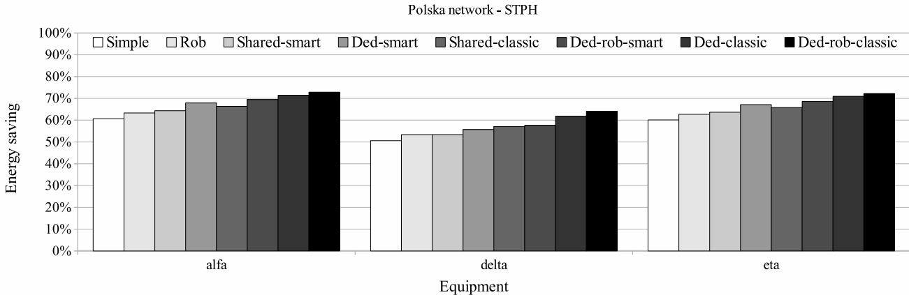
Figure 5: Energy savings achieved by STPH when implementing the different protection schemes on polksa instances.
