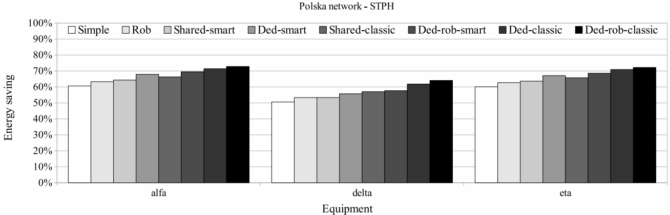
Figure 5: Energy savings achieved by STPH when implementing the different protection schemes on polksa instances.
