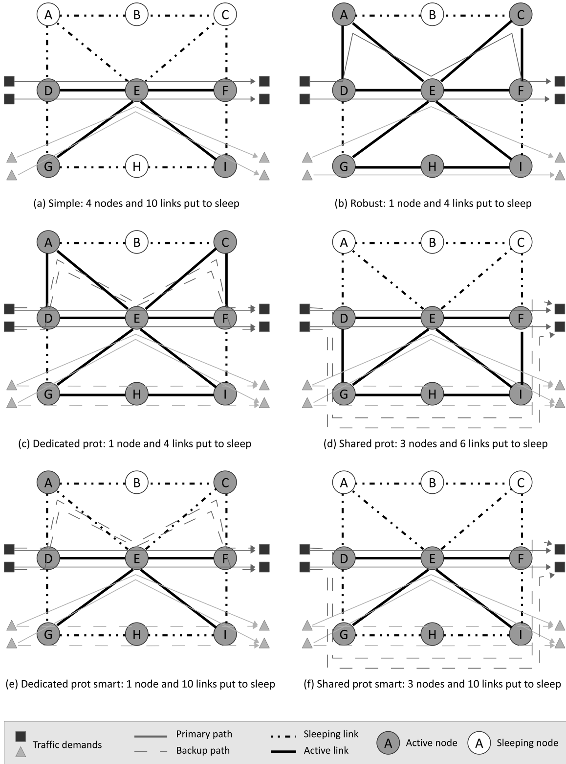
Figure 2: Energy consumption minimization vs Resilience requirements.
