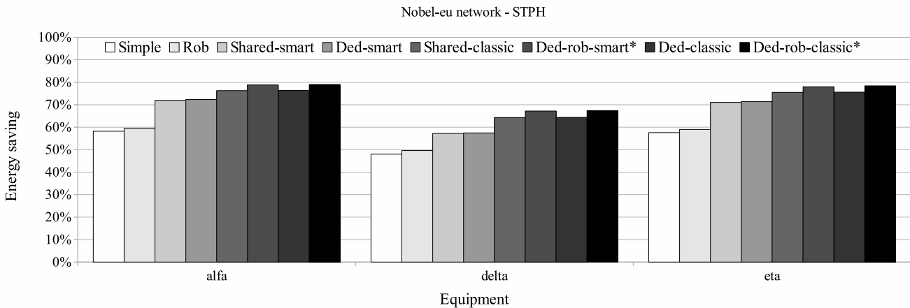
Figure 7: Energy savings achieved by STPH when implementing the different protection schemes on nobel-eu instances. The * in the graph legend is used for the instances solved, due to complexity issues, with STPH-RP using \Omega = 10 .
