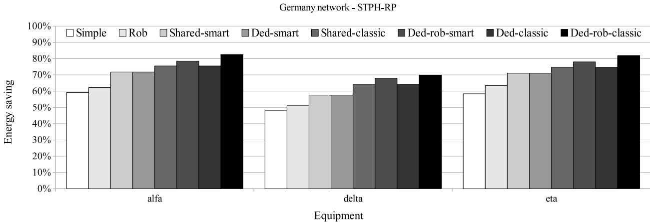
Figure 11: Energy savings achieved by STPH-RP with \Omega = 5 when implementing the different protection schemes on germany instances.
