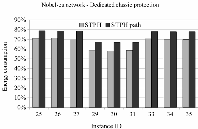
Figure 10: Energy saving comparison between STPH and STPH-RP on nobel-eu network with dedicated classic protection.
