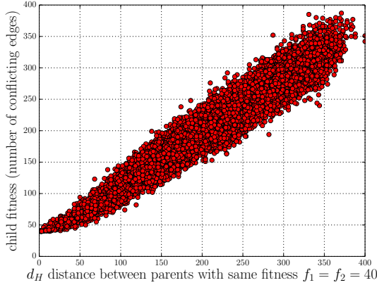
Figure 4: Each point of the chart, called child-solution, corresponds to one non-legal 48-coloring of the \langle dsjc500.5 \rangle graph; It has been produced by the GPX crossover of two other non-legal 48-colorings, called parents-solutions. Both parents are randomly generated with the same fitness value (the same number of conflicting edges). Their distance d_H in the search-space is indicated on the abscissa axis. The number of conflicting edges of the child is indicated on the ordinate axis.
