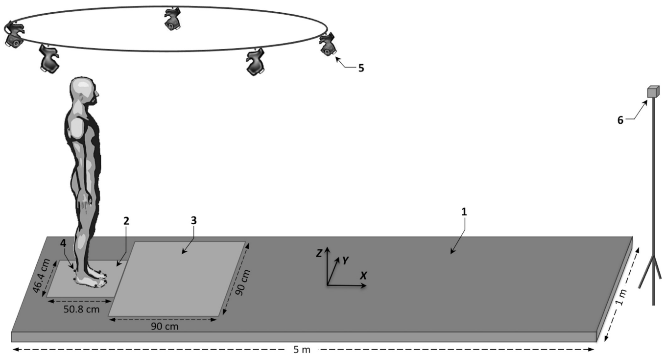
Fig. 1. Schematic illustration of the experimental set-up. Legend: (1) walkway; (2) and (3) force-plates; (4) reflective marker; (5) Vicon camera; and (6) visual target.
