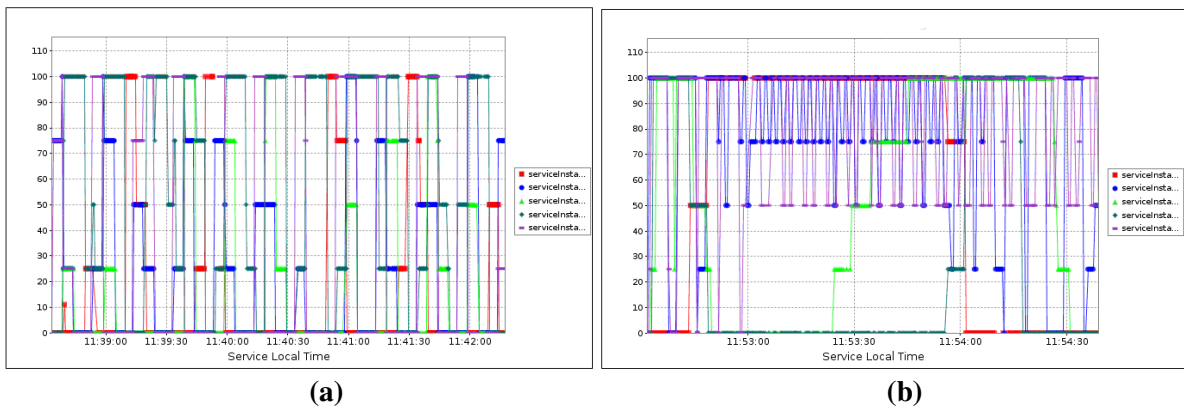
Figure 9. „Full-capacity” test – TPSI load variation in time: a) Blocking TCP; b) Non-blocking TCP (Java NIO).
