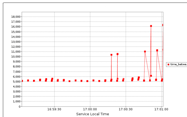
Figure 6. „Normal” test – Response time perceived by the clients (sec) using blocking TCP sockets. Similar results were obtained with non-blocking TCP sockets.
