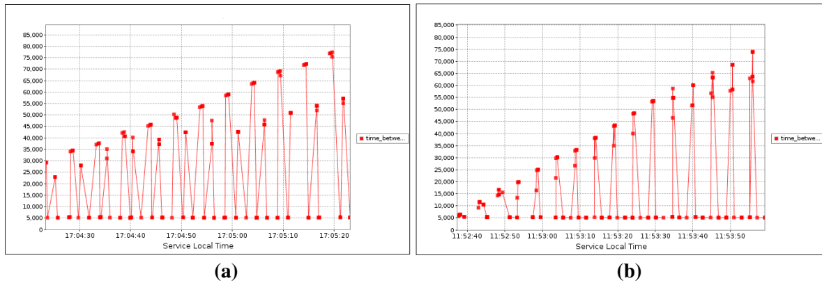
Figure 10. „Full-capacity” test – Response time perceived by the clients (sec) ): a) Blocking TCP; b) Non-blocking TCP (Java NIO).
