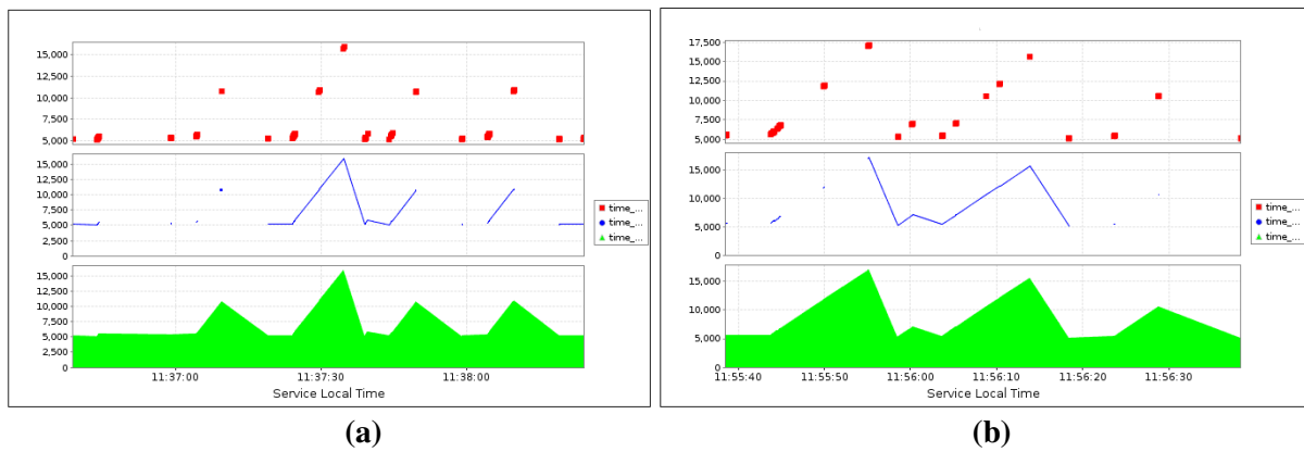
Figure 8. „Burst” test – Response time perceived by the clients (sec): a) Blocking TCP; b) Non-blocking TCP (Java NIO).
