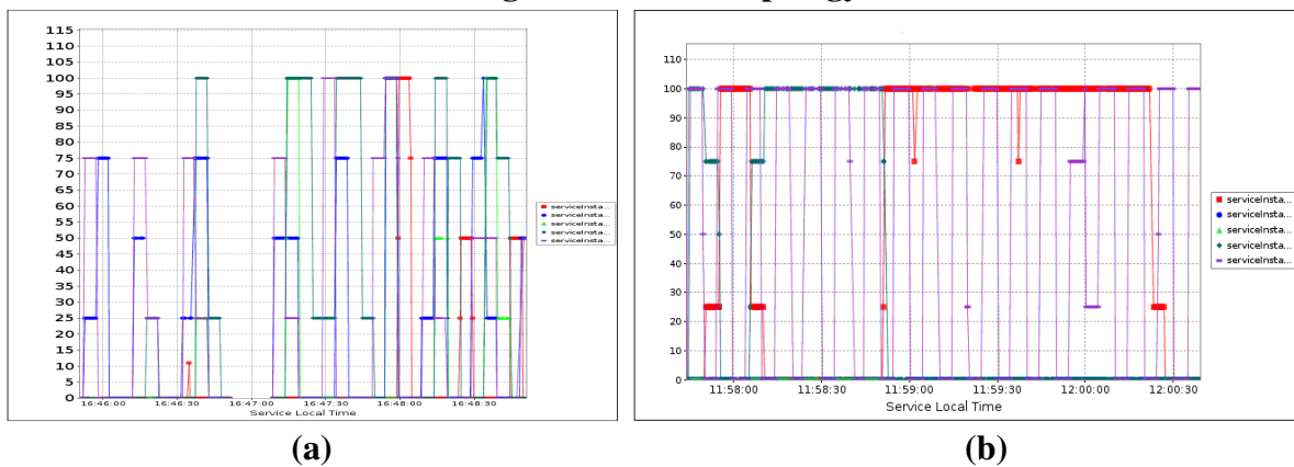
Figure 5. „Normal” test – TPSI load variation in time: a) Blocking TCP; b) Non-blocking TCP (Java NIO).
