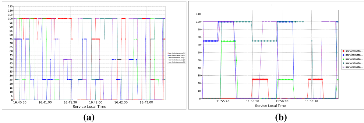
Figure 7. „Burst” test – TPSI load variation in time: a) Blocking TCP; b) Non-blocking TCP (Java NIO).
