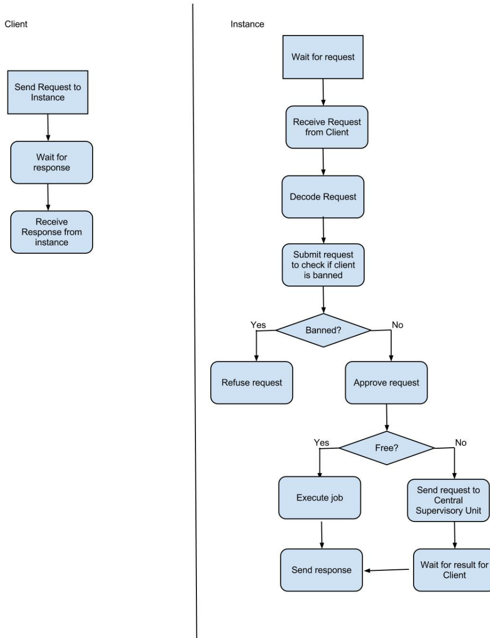
Figure 1. Client-TPSI interaction.
