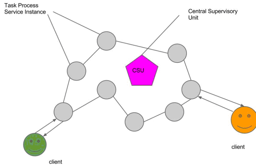
Figure 4. Service topology.
