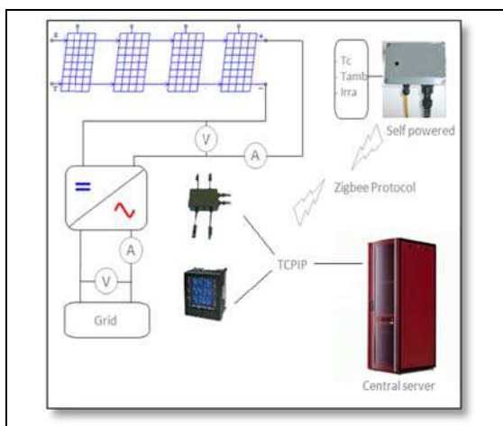
Figure 1: Monitoring system on single phase grid connected PV system
