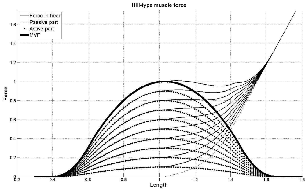
Figure 1. Force-length relations in Hill-type muscle models: Changes in activation levels are associated with a group of contractile force curves (dotted curves); the addition of passive properties (dashed curve) provides the global force-length curves (solid curves)
