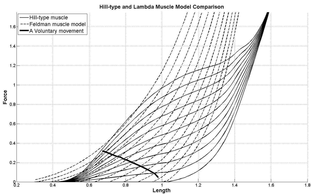
Figure 3 Comparison between the \lambda model and a Hill-type model: the bold solid path shows an example of force and length variations associated with a voluntary concentric contraction of the muscle (muscle length decreases) caused by changes in motor commands.
