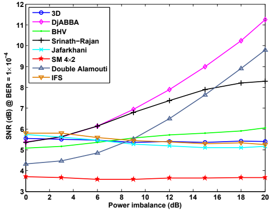
Fig. 5. Performance of distributed MIMO broadcasting using different STBCs in presence of power imbalances, soft-output sphere decoding, LDPC rate 4/9, DVB-NGH MIMO channel with f_d = 33.3\text{Hz} .
