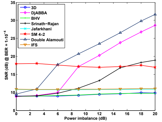
Fig. 6. Performance of distributed MIMO broadcasting using different STBCs in presence of power imbalances, soft-output sphere decoding, LDPC rate 5/6, DVB-NGH MIMO channel with f_d = 33.3\text{Hz} .
