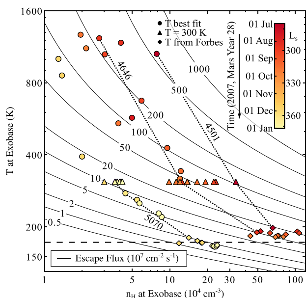
Figure 2. Best fit temperature and density for the hydrogen corona as a function of time. Parameters are shown for all 20 observations analyzed using three temperature assumptions: circles, temperature as a free parameter over the range 100–1600 K; triangles, temperature fixed at 300 K; diamonds, temperature from the empirical thermosphere model of Forbes et al. [2008]. Symbols are colored by time of observation. Contours give Jeans escape flux of hydrogen at the exobase. Dotted lines connect parameters fit to observations shown in Figure 1 for each temperature assumption, identified by orbit number. These lines demonstrate the anticorrelation of model fitted temperature and density. Dashed line indicates the exobase temperature for which the effusion velocity from the exobase is equal to the thermospheric diffusion velocity. Independent of exobase temperature, we observe a nearly uniform order of magnitude decrease in the escape flux of hydrogen at the exobase of Mars over 6 months in the fall of 2007.
