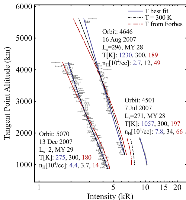
Figure 1. Atmospheric airglow observations and model with three temperature assumptions. Gray points represent observed Lyman alpha airglow intensity in kiloRayleighs ( 1 \text{ kR} = 10^9/4\pi \text{ photons/cm}^2/\text{ster/s} ) and associated uncertainties (see text) as a function of minimum altitude along instrument line of sight (tangent point altitude) for three observations. Curves represent best fit model output for three different temperature assumptions: solid blue, best fit model temperature in the range 100–1600 K; short dash-dotted black, temperature fixed at 300 K; long dash-dotted red, temperature from the empirical thermosphere model of Forbes et al. [2008]. Profiles are annotated with observation orbit number, date, and best fit temperature and density for each temperature assumption in the order listed above. The model accurately reproduces observed brightness with a single population across a wide range of observations. Observations are in time sequence from right to left, demonstrating the decrease in hydrogen corona brightness observed in Fall 2007.
