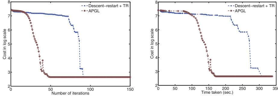
FIG. 6.8. A large-scale instance of rank 5 completion of 50000 \times 50000 matrix with OS = 8 . \lambda = 2\|\mathbf{W} \odot \mathbf{X}\|_{op}/10^5 as suggested in [39]. The proposed framework is competent for very low ranks and when a high accuracy is sought. However, we spend considerable time in just traversing through ranks before arriving at the optimal rank.
