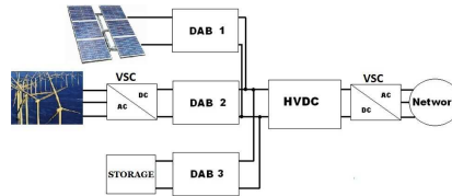
Figure 10: HVDC network
