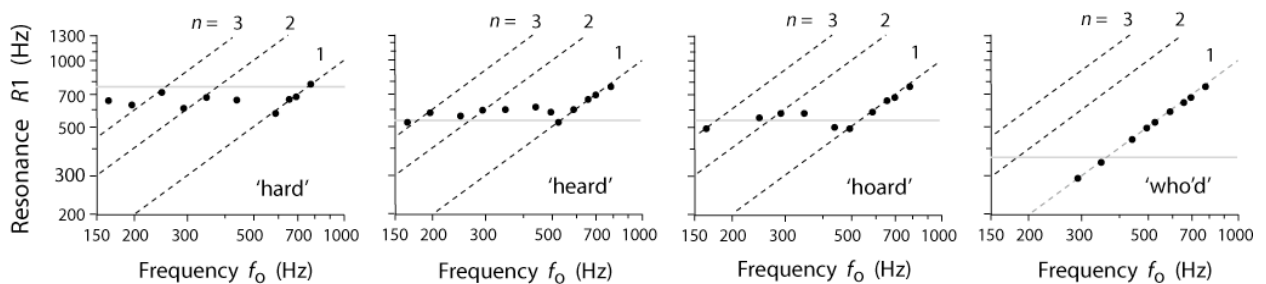
Figure 4. Examples of an alto starting to use R1:f_0 tuning when f_0 approaches the value of R1 for that vowel in speech. The dashed diagonal lines indicate the relationships R1 = nf_0 . The horizontal grey lines indicate the value of R1 measured for the same singer and vowel in speech.
