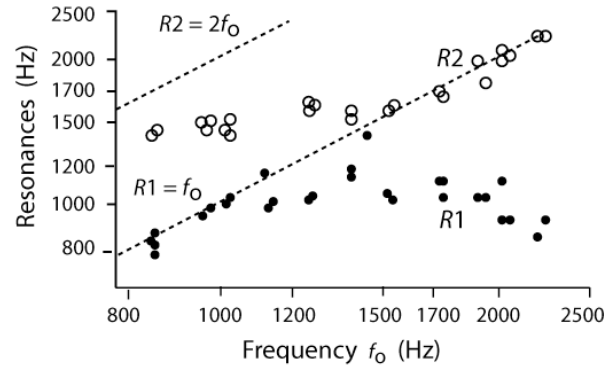
Figure 3. Example of a soprano switching from R1:f_0 to R2:f_0 tuning at extremely high pitch once R1 can no longer be increased. The dashed diagonal lines indicate the relationships R1 = f_0 , R2 = f_0 and R2 = 2f_0 . The measured frequencies of R1 and R2 are indicated by closed and open circles respectively.
