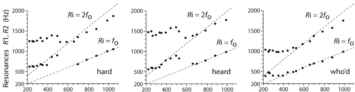
Figure 6. Example of a soprano using R1:2f_0 tuning at low pitch. She then switches to simultaneous R1:f_0 and R2:2f_0 tuning. The dashed diagonal lines indicate the relationships R_i = n f_0 .
