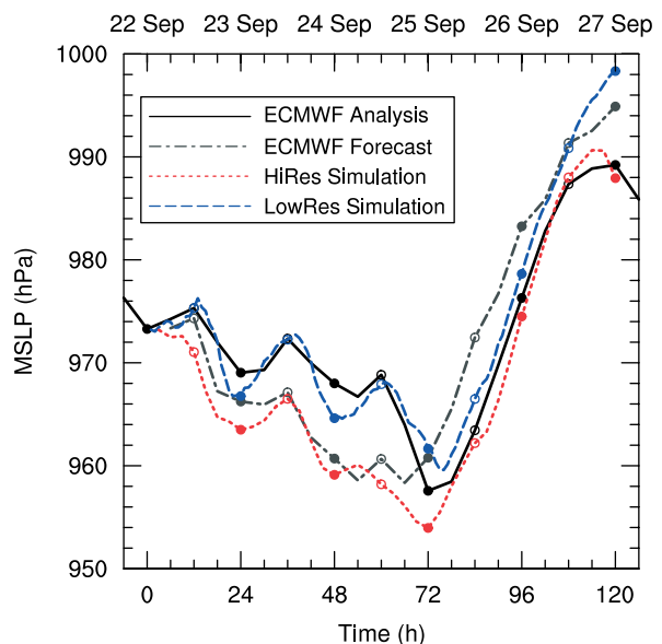
Figure 4. Temporal evolution of the MSLP minimum of Helene from 0000 UTC 22 September 2006, in the ECMWF analysis and operational forecast, and in Meso-NH HiRes and LowRes runs. Filled circles at 0000 UTC and hollow circles at 1200 UTC. This figure is available in colour online at wileyonlinelibrary.com/journal/qj
