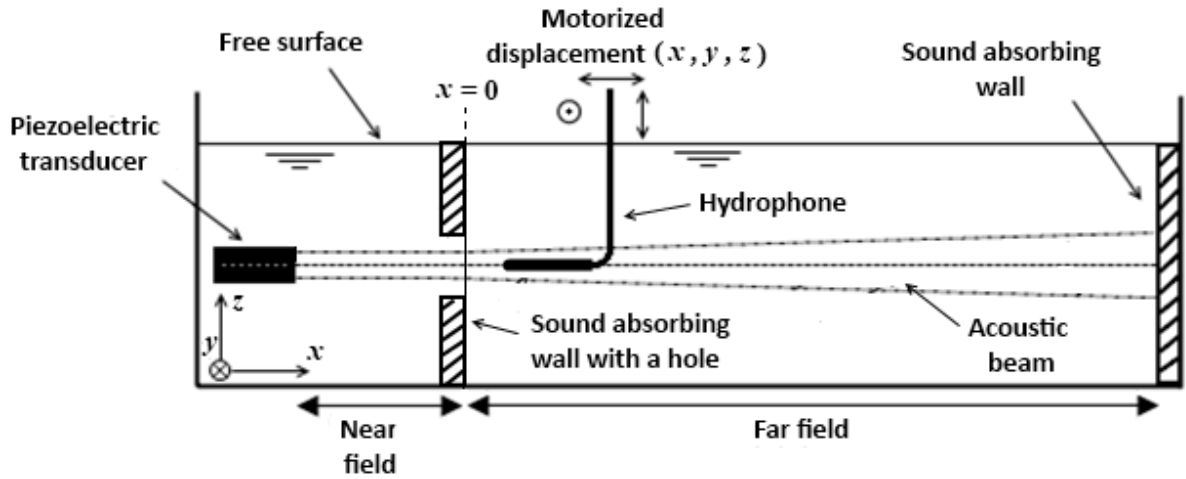
Figure 1: Experimental configuration (side view); the sound-absorbing wall with the hole is covered with a plastic film to impose a no-slip boundary condition for the hydrodynamic flow. The origin of the coordinates (x,y,z) is chosen at the center of this hole. The domain of investigation, situated on the right hand side of the absorbing wall with a hole ( x > 0 ) is 16 cm deep, 18 cm wide and 47 cm long.
