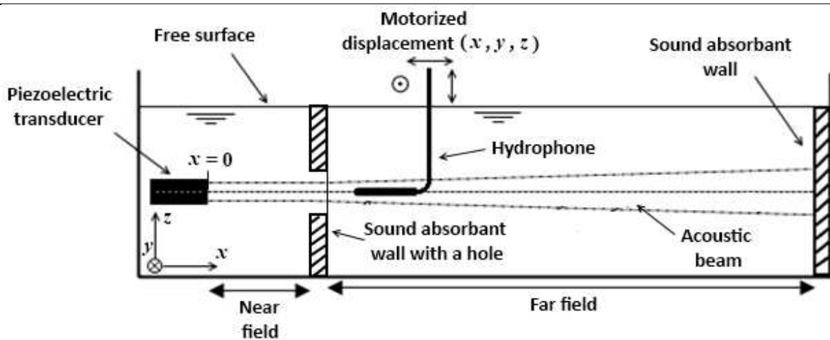
Figure 1: Experimental configuration (side view); the sound-absorbant wall with the hole is covered with a plastic film to impose a no-slip boundary condition for the hydrodynamic flow. The origin of the frame is chosen at the center of this hole. The domain of investigation, situated on the right hand side of the absorbing wall with a hole ( x > 0 ) is 16 \text{ cm} deep, 18 \text{ cm} wide and 47 \text{ cm} long.
