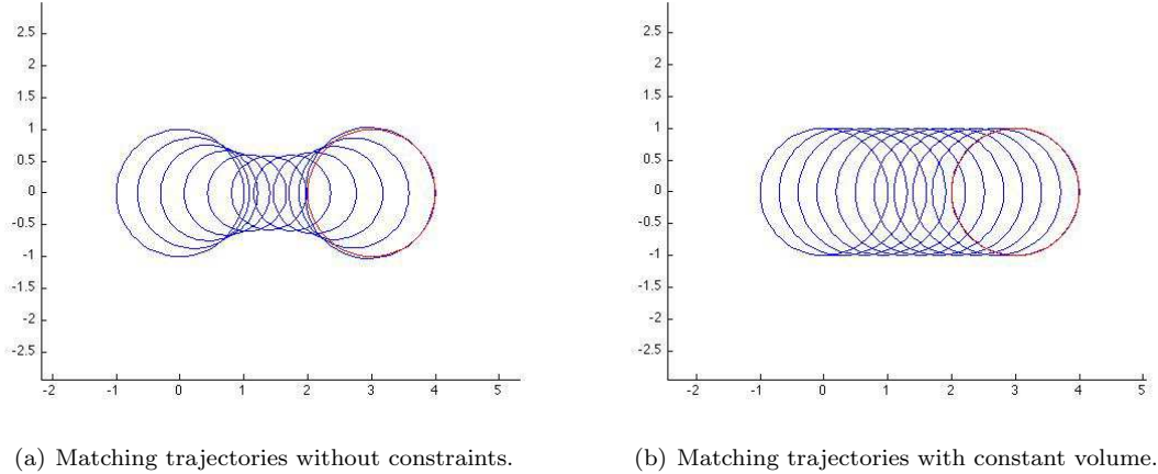
Figure 1: Matching trajectories.
