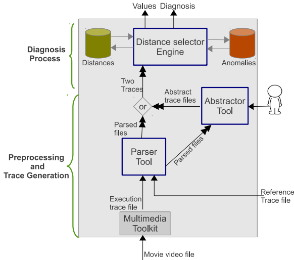
Fig. 2. TED Architecture
