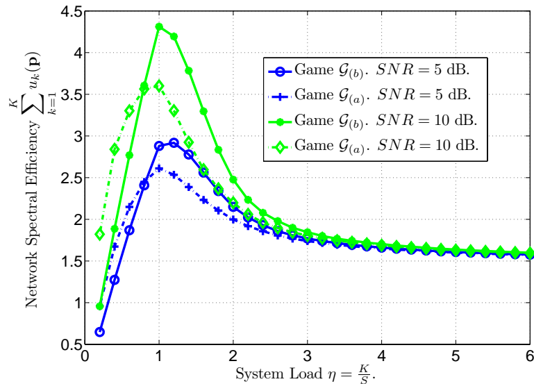
Fig. 7. Network spectral efficiency as a function of the system load \eta = \frac{K}{S} for different SNR = \frac{p_{\max}}{\sigma^2} levels in dBs.
