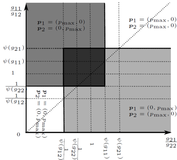
Fig. 4. Nash equilibrium action profiles as a function of the channel ratios \frac{g_{11}}{g_{12}} and \frac{g_{21}}{g_{22}} for the two-player-two-channel game \mathcal{G}_{(b)} , respectively. The function \psi : \mathbb{R}_+ \rightarrow \mathbb{R}_+ is defined as follows: \psi(x) = 1 + \text{SNR } x . The best response function \text{BR}_k(\mathbf{p}_{-k}) , for all k \in \mathcal{K} , is defined by (12). Here, it has been arbitrarily assumed that \psi(g_{11}) < \psi(g_{21}) .
