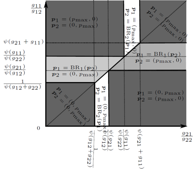
Fig. 2. Nash equilibrium action profiles as a function of the channel ratios \frac{g_{11}}{g_{12}} and \frac{g_{21}}{g_{22}} for the two-player-two-channel game \mathcal{G}_{(a)} . The function \psi : \mathbb{R}_+ \rightarrow \mathbb{R}_+ is defined as follows: \psi(x) = 1 + \text{SNR}x . The best response function \text{BR}_k(\mathbf{p}_{-k}) , for all k \in \mathcal{K} , is defined by (12). Here, it has been arbitrarily assumed that \frac{\psi(g_{21})}{\psi(g_{12})} < \frac{\psi(g_{11})}{\psi(g_{22})} .
