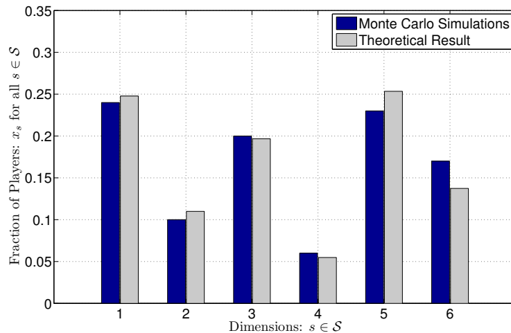
Fig. 9. Fraction of players transmitting over channel s , with s \in \mathcal{S} , calculated using Monte-Carlo simulations and using Eq. (26) for a network with S = 6 channels, K = 60 players, with \mathbf{b} = (b_s)_{\forall s \in \mathcal{S}} = (0.25, 0.11, 0.20, 0.05, 0.25, 0.14) , and \text{SNR} = 10 \log_{10} \left( \frac{p_{\max}}{N_0 B} \right) = 10 dB.
