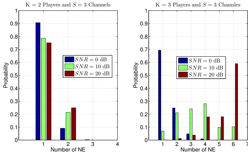
Fig. 6. Probability of observing a specific number of NE in the game \mathcal{G}_{(b)} calculated using Monte-Carlo simulations.
