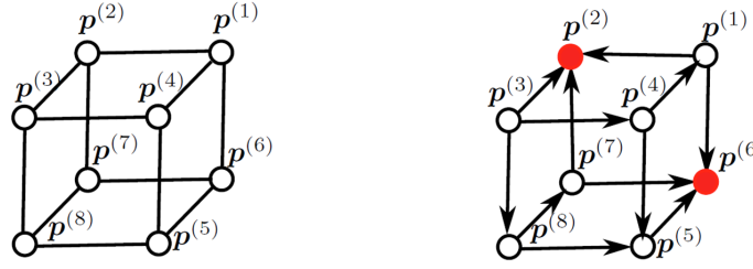
Fig. 1. (a) Non-oriented graph and (b) oriented graph representing the game \mathcal{G}_{(b)} with K = 3 , S = 2 , under the condition \phi(\mathbf{p}^{(2)}) > \phi(\mathbf{p}^{(6)}) > \phi(\mathbf{p}^{(1)}) > \phi(\mathbf{p}^{(5)}) > \phi(\mathbf{p}^{(4)}) > \phi(\mathbf{p}^{(7)}) > \phi(\mathbf{p}^{(8)}) > \phi(\mathbf{p}^{(3)}) . Total number of vertices: S^K = 8 , number of neighbors per vertex: K(S - 1) = 3 . Maximum Number of NE: 4. Number of NE: 2 (red vertices in (b)).
