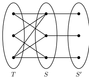
Figure 9: Example of an SC2-graph.
