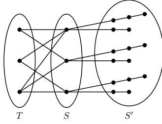
Figure 8: Example of an SC1-graph.
