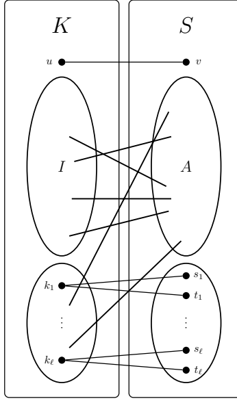
Figure 2: Reduction from MIN DISCRIMINATING CODE to MIN ID CODE (with \ell = 2\lceil \log_2(|A| + 1) \rceil ).
