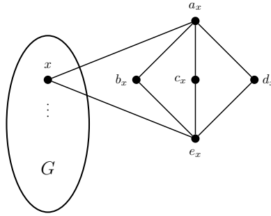
Figure 6: Reduction from MIN DOMINATING SET to MIN ID CODE.
