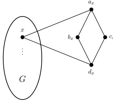
Figure 7: Reduction from MIN DOMINATING SET to MIN LOC-DOM SET.
