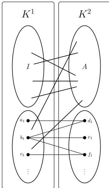
Figure 3: Reduction from MIN DISCRIMINATING CODE to MIN ID CODE (with \ell = \lceil \log_2(|A| + 1) \rceil ).
