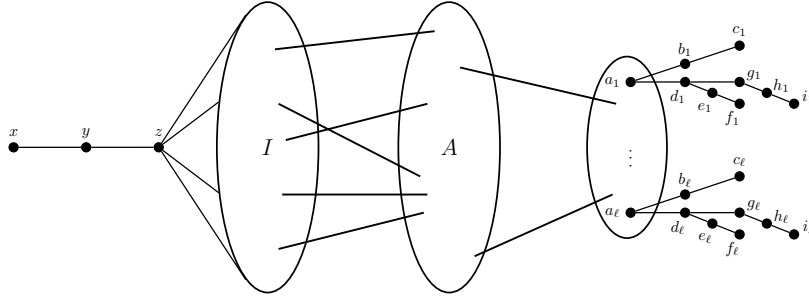
Figure 1: Reduction from MIN DISCRIMINATING CODE to MIN ID CODE (with \ell = \lceil\log_2(|A| + 1)\rceil ).
