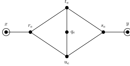
Figure 5: Reduction gadget for edge e = \{x, y\} in Reduction 28 from MIN VERTEX COVER to MIN LOC-DOM SET. The original vertices of G , x and y , are circled.
