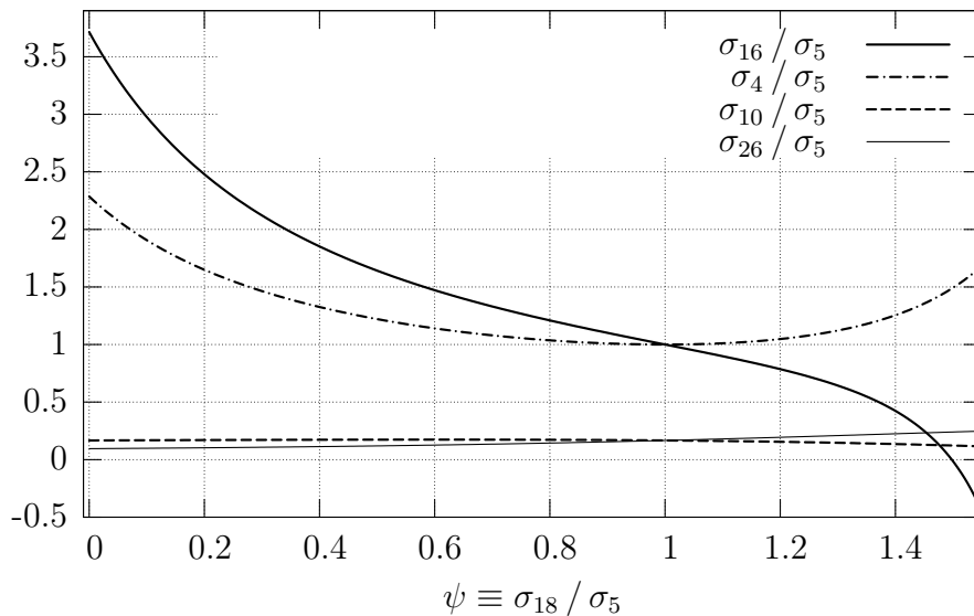
Figure 1. Fourth order isotropy parameters for the D3Q27 lattice Boltzmann scheme.
