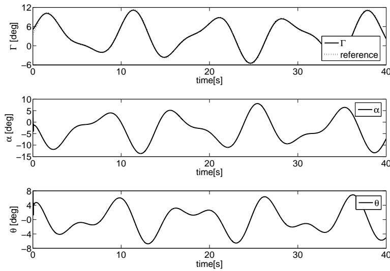
Figure 13 Trajectory tracking.
