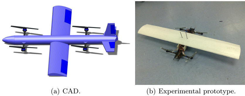
Figure 1 Quad-Tilting Rotor Convertible UAV.
