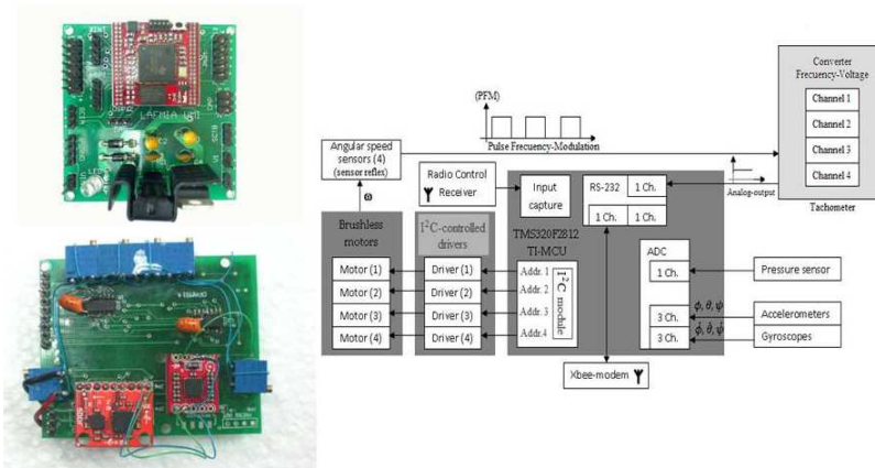
Figure 15 Homemade IMU, DSP-based embedded flight system and working principle of the Quad-plane UAV system.
