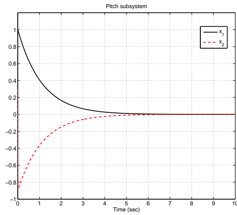
Figure 1.14: Response of the Pitch control loop
