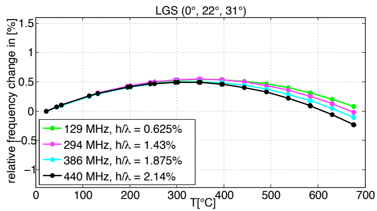
Fig. 4. Experimental frequency-temperature laws of (0^\circ, 22^\circ, 31^\circ) LGS cut
