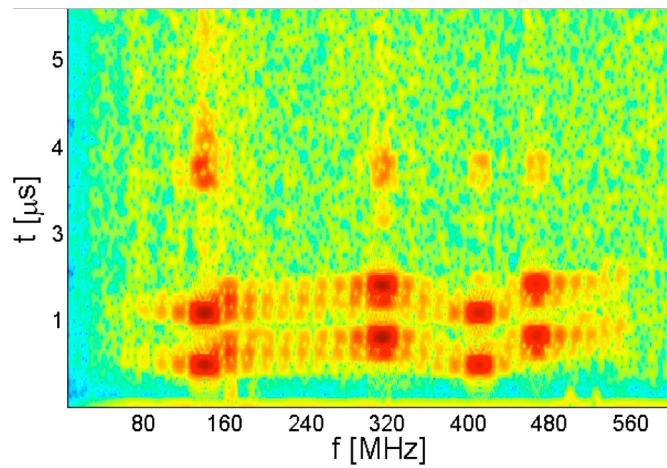
Fig. 12. Spectrogram of R-SAW (0°, 138.5°, 26.7°) LGS cut at 440°C.
