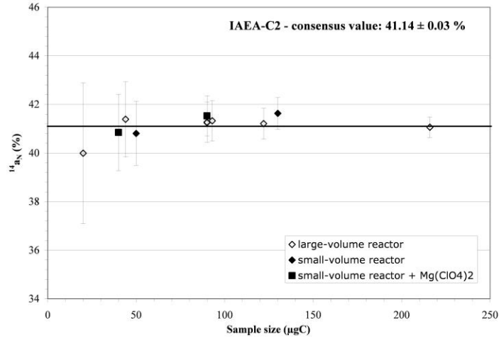
Figure 5 The normalized ^{14}\text{C} concentration ratio of IAEA-C2 as a function of sample size.
