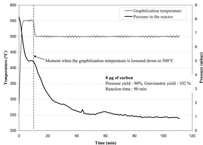
Figure 3 Graphitization curves for a sample containing 8 µg of carbon in the small-volume reactor with the Mg(ClO 4 ) 2 trap. When the reduction temperature is changed from 550 to 500 °C, the pressure drops again. The reaction time is the time needed to obtain a plateau in the pressure curve.
