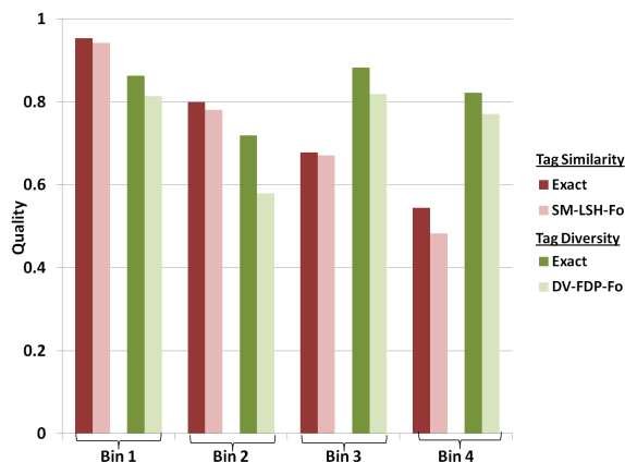
Figure 8: Quality: Varying Tagging Tuples
