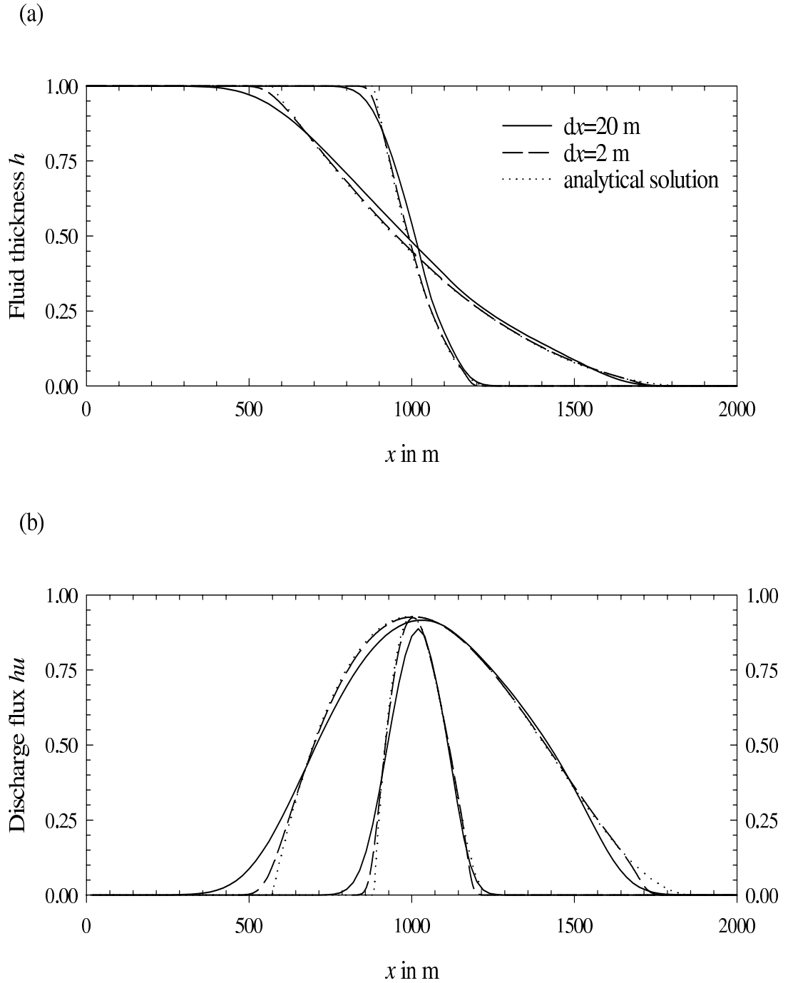
Figure 5: (a) Fluid thickness h and (b) discharge flux hu versus distance, obtained for \delta = 0^\circ and \theta = 0^\circ at time t = 37 s and t = 137 s , calculated with the analytical solution (dotted lines) and with the numerical model for dx = 20 m (solid lines) and dx = 2 m (dashed lines).
