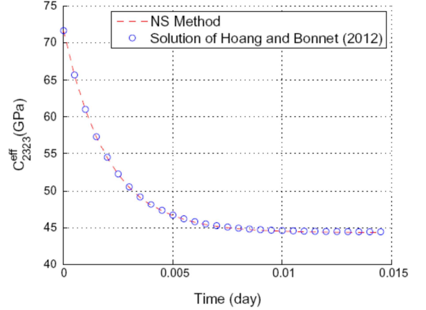
Fig. 6. Component C_{2323}^{\text{eff}}(t) as a function of time, determined by the NS method and by the FFT approximate solution of Hoang-Duc and Bonnet (2012).
