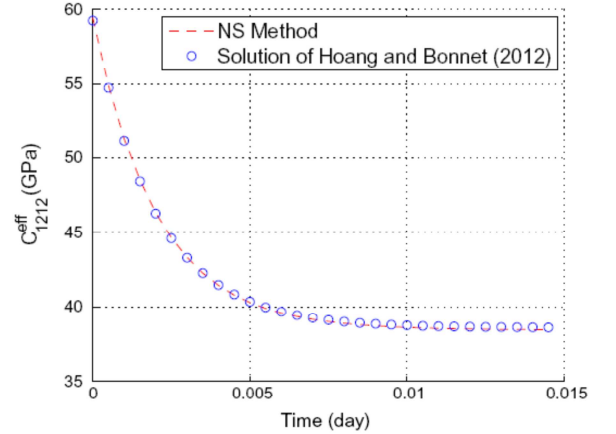
Fig. 7. Component C_{1212}^{\text{eff}}(t) as a function of time, determined by the NS method and by the FFT approximate solution of Hoang-Duc and Bonnet (2012).
