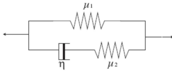
Fig. 4. Viscoelastic rheological scheme of Zener's type.
