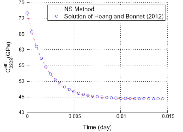
Fig. 6. Component C_{2323}^{eff}(t) as a function of time, determined by the NS method and by the FFT approximate solution of Hoang-Duc and Bonnet (2012).
