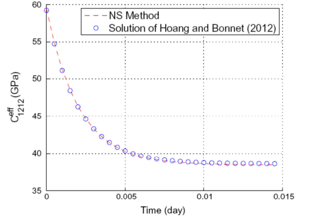
Fig. 7. Component C_{1212}^{eff}(t) as a function of time, determined by the NS method and by the FFT approximate solution of Hoang-Duc and Bonnet (2012).
