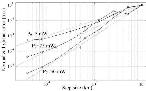
Figure 2: Experimental convergence curve (logarithmic scale) for the S3F-RK4 method applied for solving the GNLSE on the test example with different peak-power values (solid lines). The convergence order is ranging from 2 to 4 depending on the importance of Kerr nonlinearity (theoretical curves in dotted lines).
