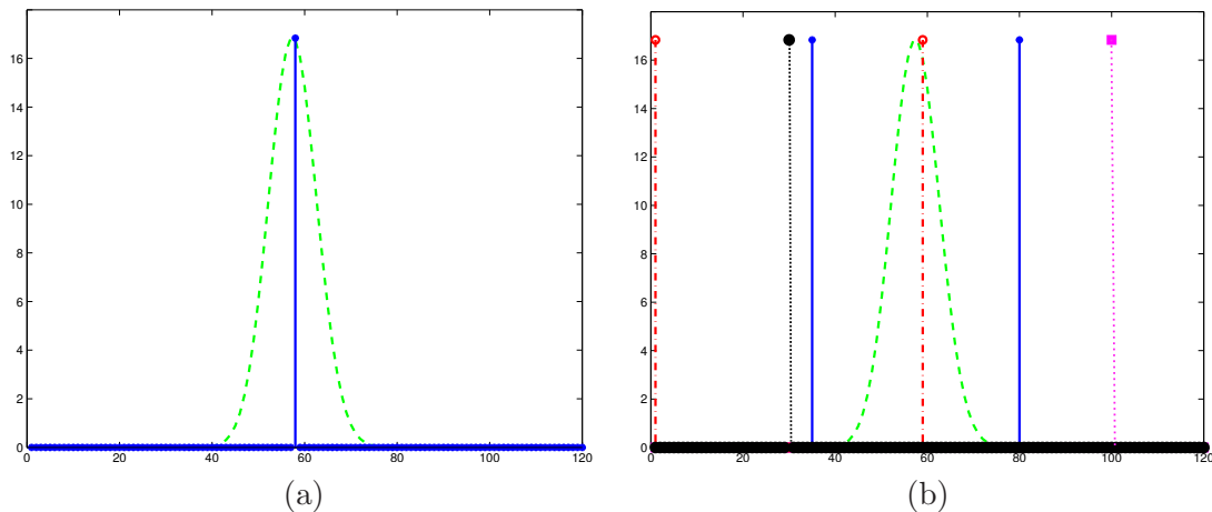
Figure 1: Approximation bounds for a = 100 , b = 30 and \sigma^2 = 50 : (a) Approximation n^* from (35) (solid blue) to the maximizer of function n \mapsto \Pi(a, b, n) (dashed green), (b) function n \mapsto \Pi(a, b, n) (dashed green), summation bounds resulting from (34) with \Delta = 3 (solid blue) and from [9, 51] (dash-dotted red). The values of a and b are indicated with black and magenta dotted lines, respectively.
