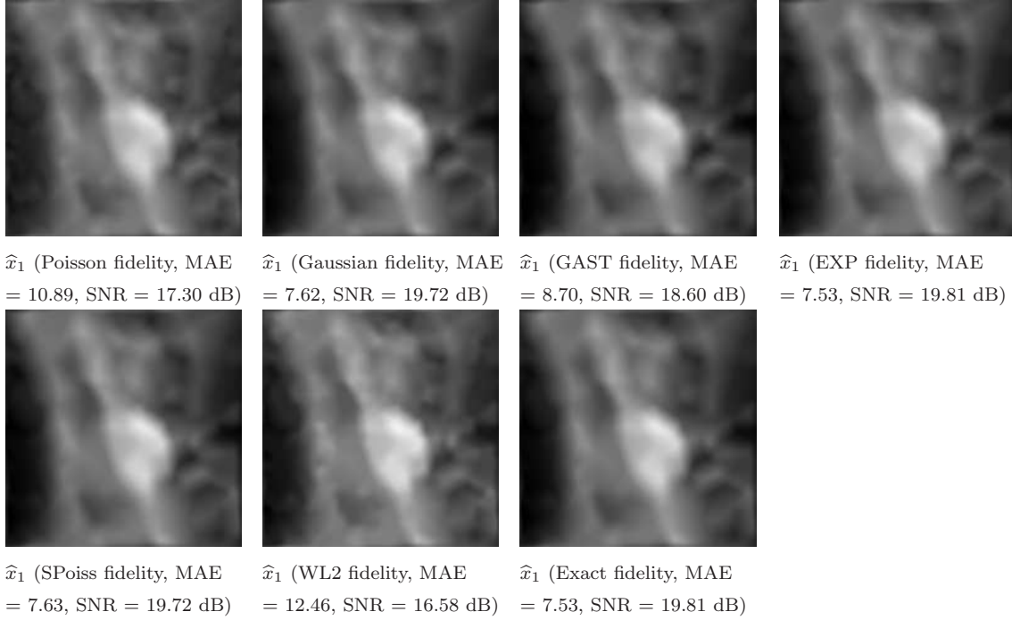
Figure 3: Restoration results of image \bar{x}_1 for TV+Hessian regularization strategy and several choices for the data fidelity term.
