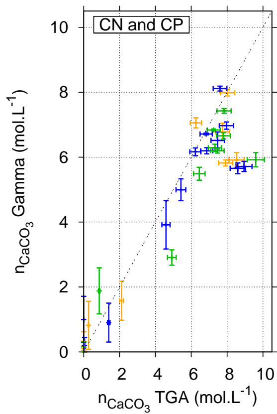
Figure 16: Comparison between n_{\text{CaCO}_3} obtained by TGA-MS and by GRAM.
