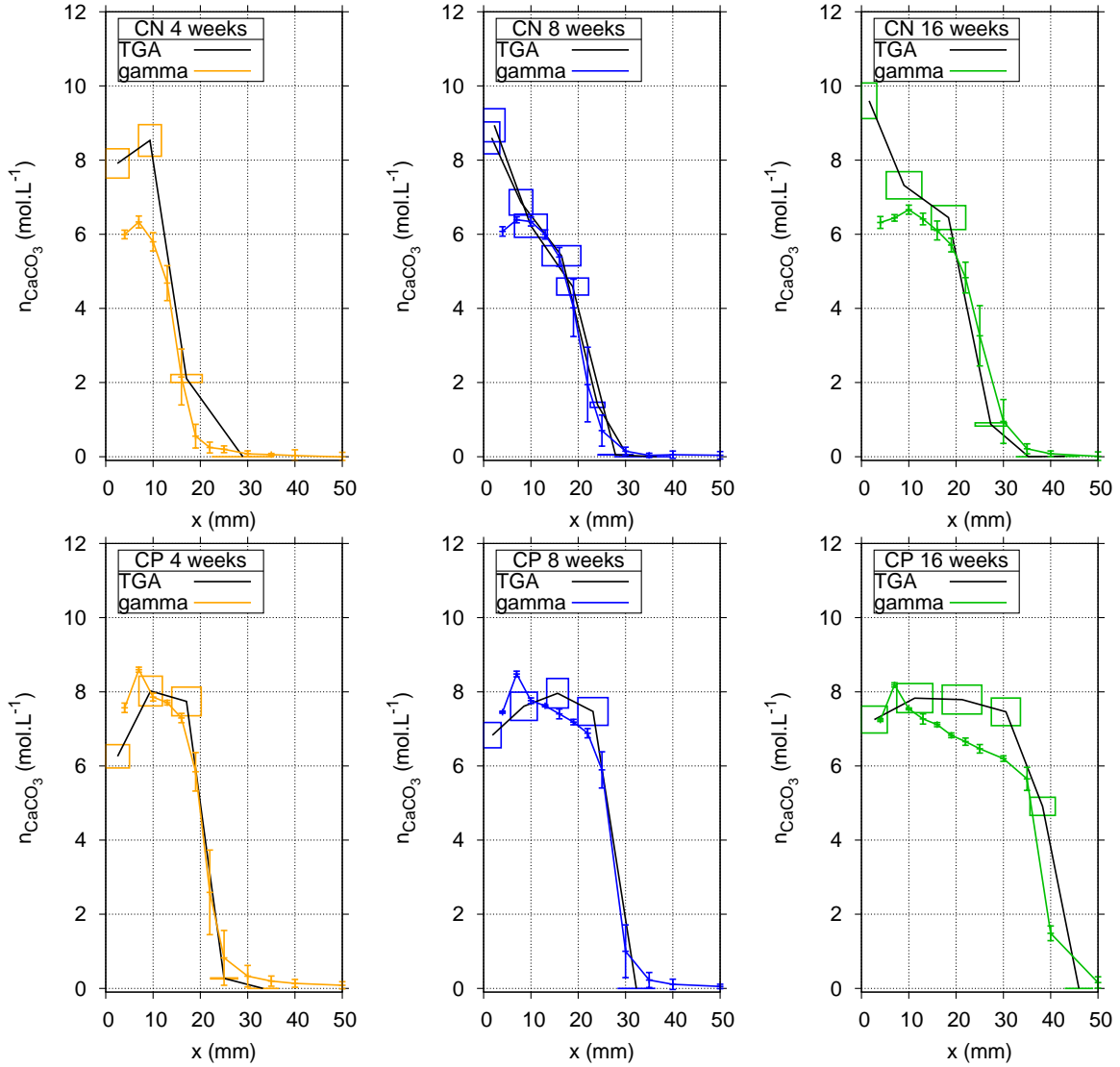
Figure 15: Assessment of CO 2 fixed to the cement matrix as \overline{C\overline{C}} ( n_{\overline{C\overline{C}}} ) for CN and CP after 4 (orange), 8 (blue) and 16 (green) weeks of accelerated carbonation. TGA-MS data are represented by coloured boxes while GRAM data are represented as coloured lines.
