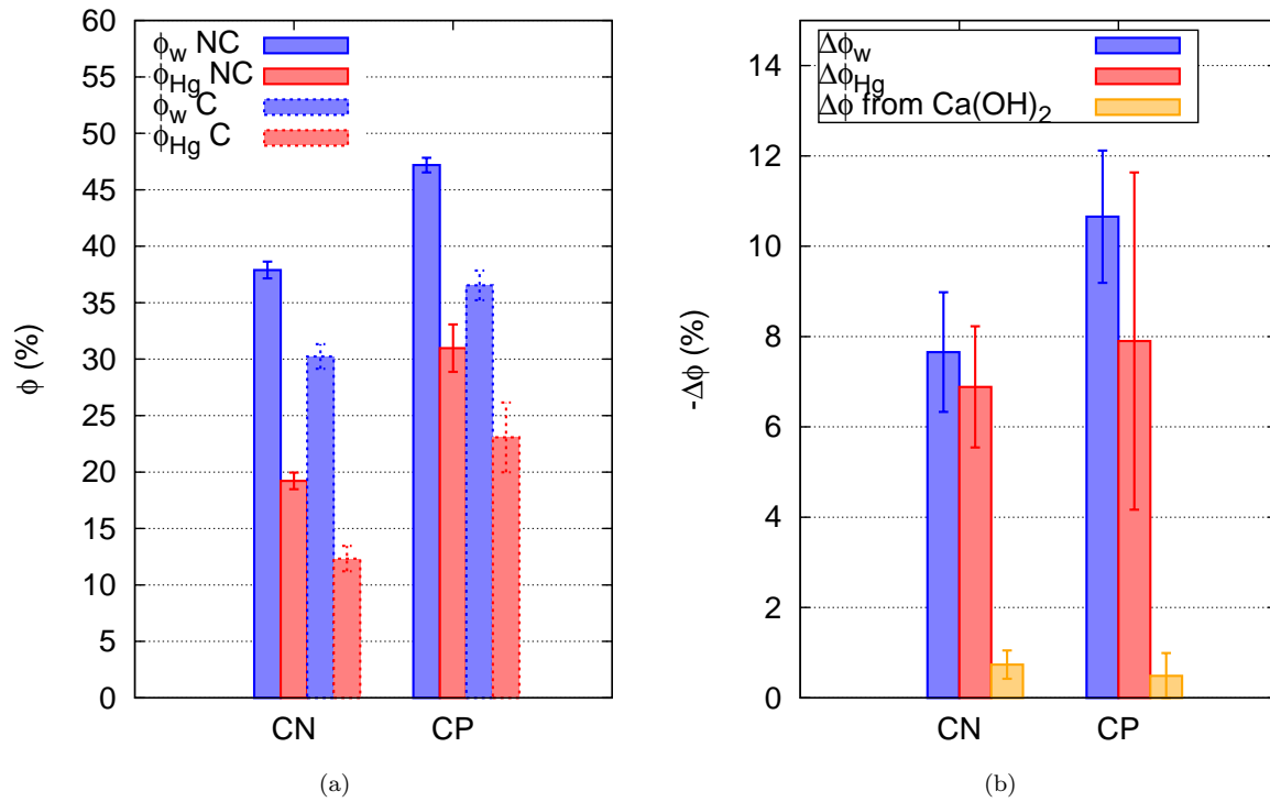
Figure 18: Fig. (a) represents total porosity measured by MIP \phi_{Hg} , total porosity measured by GRAM \phi_w , for carbonated (C) and non-carbonated (NC) cement pastes is presented. Fig. (b) represents the variation of porosity between a non-carbonated state and a totally carbonated state for both MIP and GRAM. While the porosity is different, the porosity variation is equivalent. It is also presented the porosity variation only due to CH carbonation (see Eq. 12).
