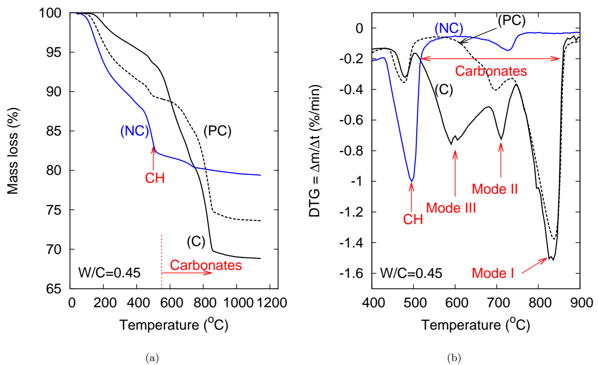
Figure 5: a/ Mass loss during a TGA experiment on fully carbonated (C), partially carbonated (PC) and non-carbonated (NC) samples (cement paste w/c = 0.45 ). b/ Derivative of the mass loss vs. temperature (DTG) in the temperature range corresponding to the decomposition of CH and \text{CC} .
