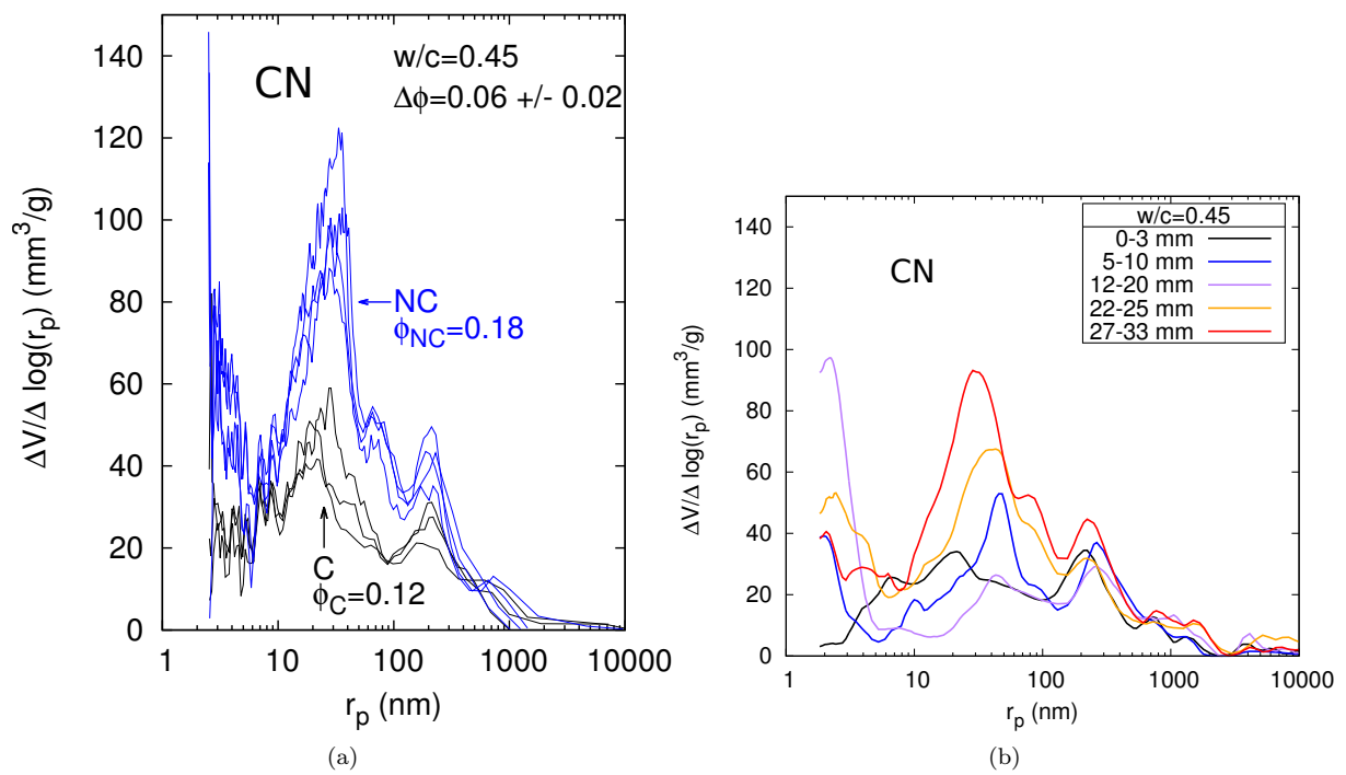
Figure 20: In Fig. (a), MIP allows us to characterize the pore size distribution in carbonated (C) and in non-carbonated (NC) samples for CN. The variability of the results is presented for various specimen. The PSD is plotted in Fig. (b) for one specimen saw at various depths which represents different carbonation stages.
