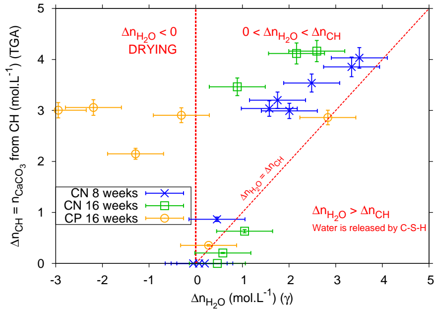
Figure 24: Molar content of water released along the profile (GRAM) after 56 and 112 days of carbonation has been extracted, and is linked to the carbonated amount of CH determined by TGA.
