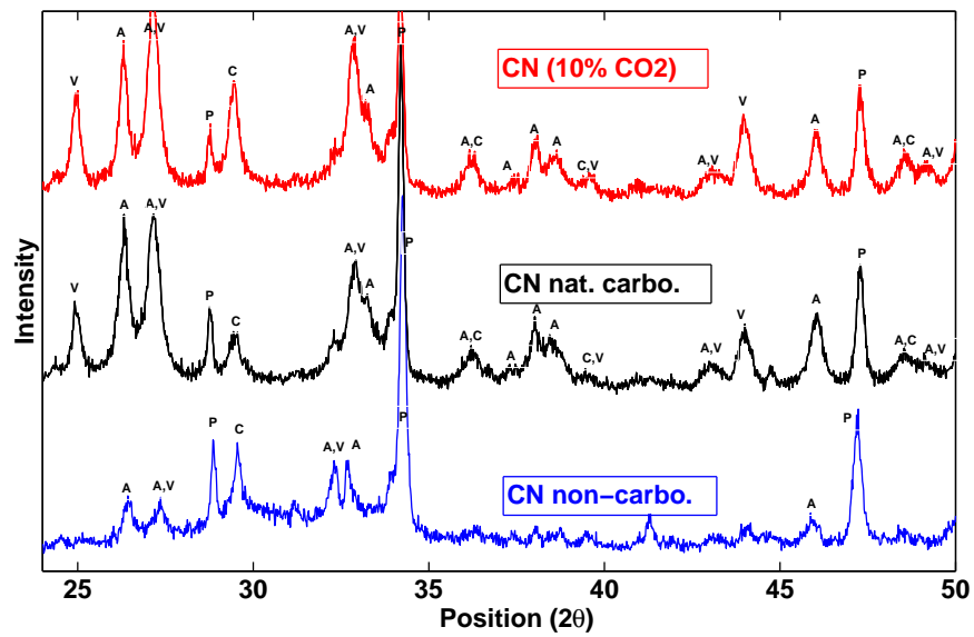
Figure 12: Comparison of XRD patterns for non-carbonated and carbonated (natural conditions and \text{CO}_2=10\% ) CN samples. A for aragonite, V for vaterite, C for calcite and P for portlandite.
