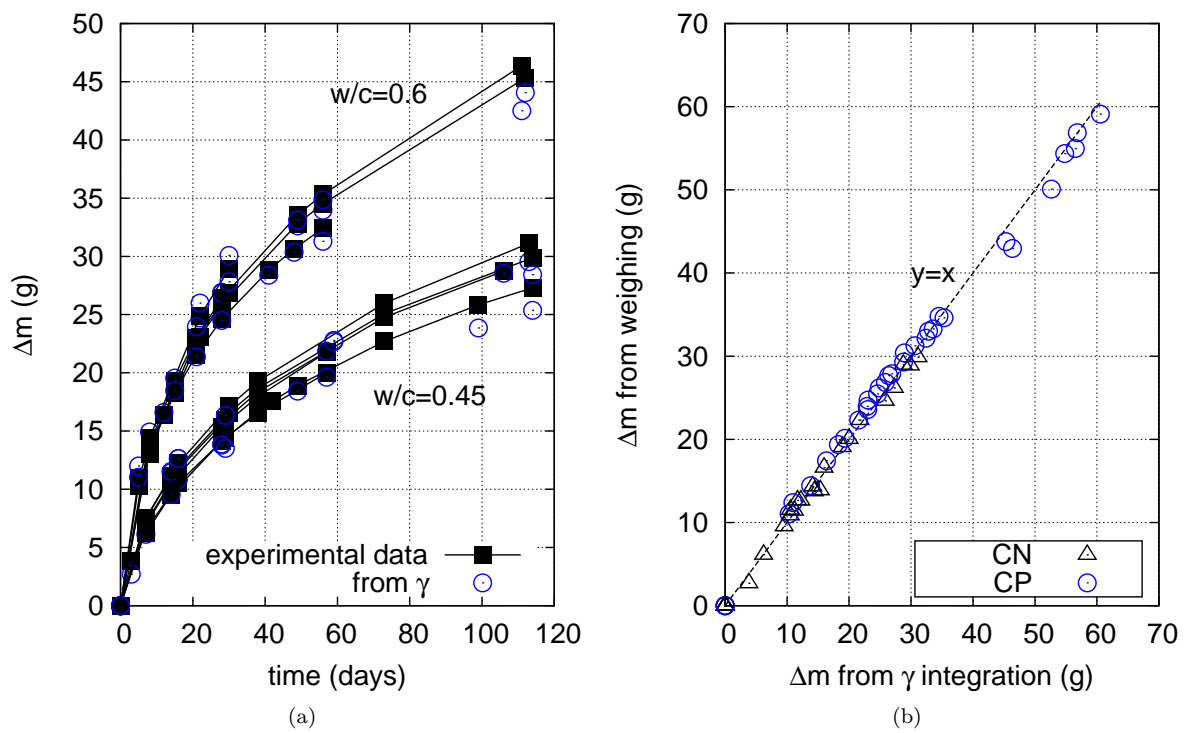
Figure 7: Two ways to assess the variation of the global mass of the specimen: integration of GRAM profiles and simple weighing of the mass gain from GRAM. Fig. (a) shows \Delta m from both methods and GRAM profile integration vs. time while Fig. (b) shows that both methods perfectly match in a y = x representation.
