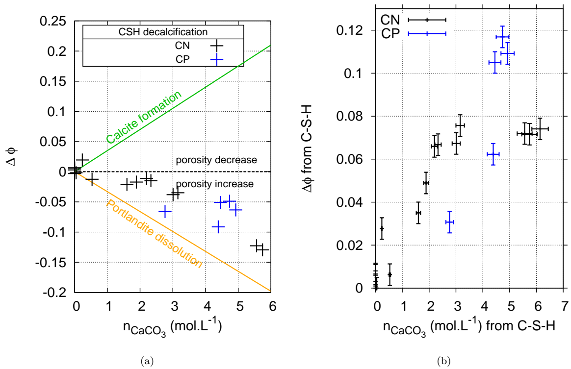
Figure 21: Fig. (a) shows each contribution for each chemical: mechanism, mainly calcium carbonate formation (chosen here as calcite), CH dissolution and C-S-H decalcification. In Fig. (b), the porosity variation for C-S-H is illustrated as a function of calcium carbonate coming from C-S-H decalcification.
