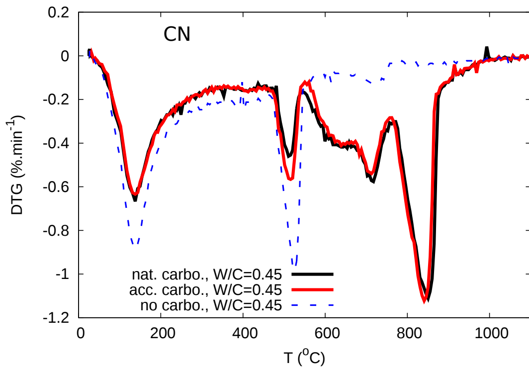
Figure 11: Comparison of DTG diagrams between non-carbonated and carbonated CN (10% \text{CO}_2 or natural carbonation).
