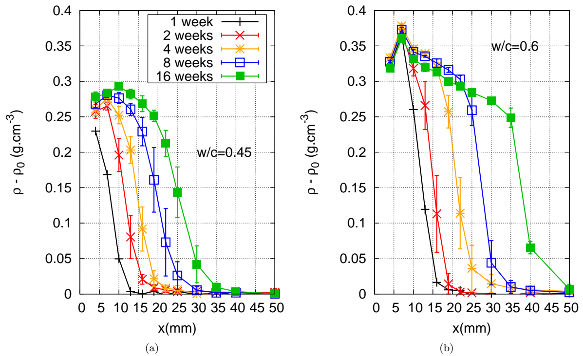
Figure 6: GRAM profiles on both CN ( w/c=0.45 , a) and CP ( w/c=0.6 , b) cement pastes. This figure shows the increase of density measured after 1, 2, 4, 8 and 16 weeks of exposure inside the incubator.
