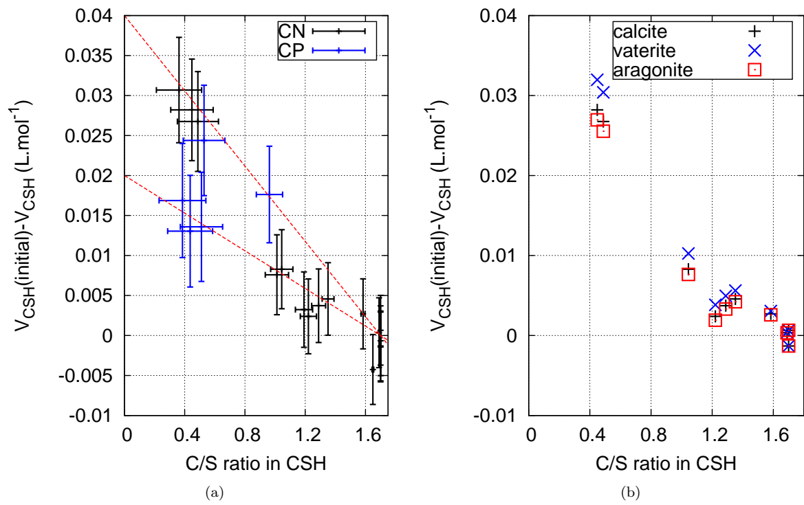
Figure 22: (a) C-S-H molar volume variation as a function of C/S for both CN and CP. (b) influence of the choice of V_{\text{C}\bar{\text{C}}}^{\text{CSH}} , results obtained for various polymorphic forms of \text{C}\bar{\text{C}} from C-S-H plotted only for CN.
