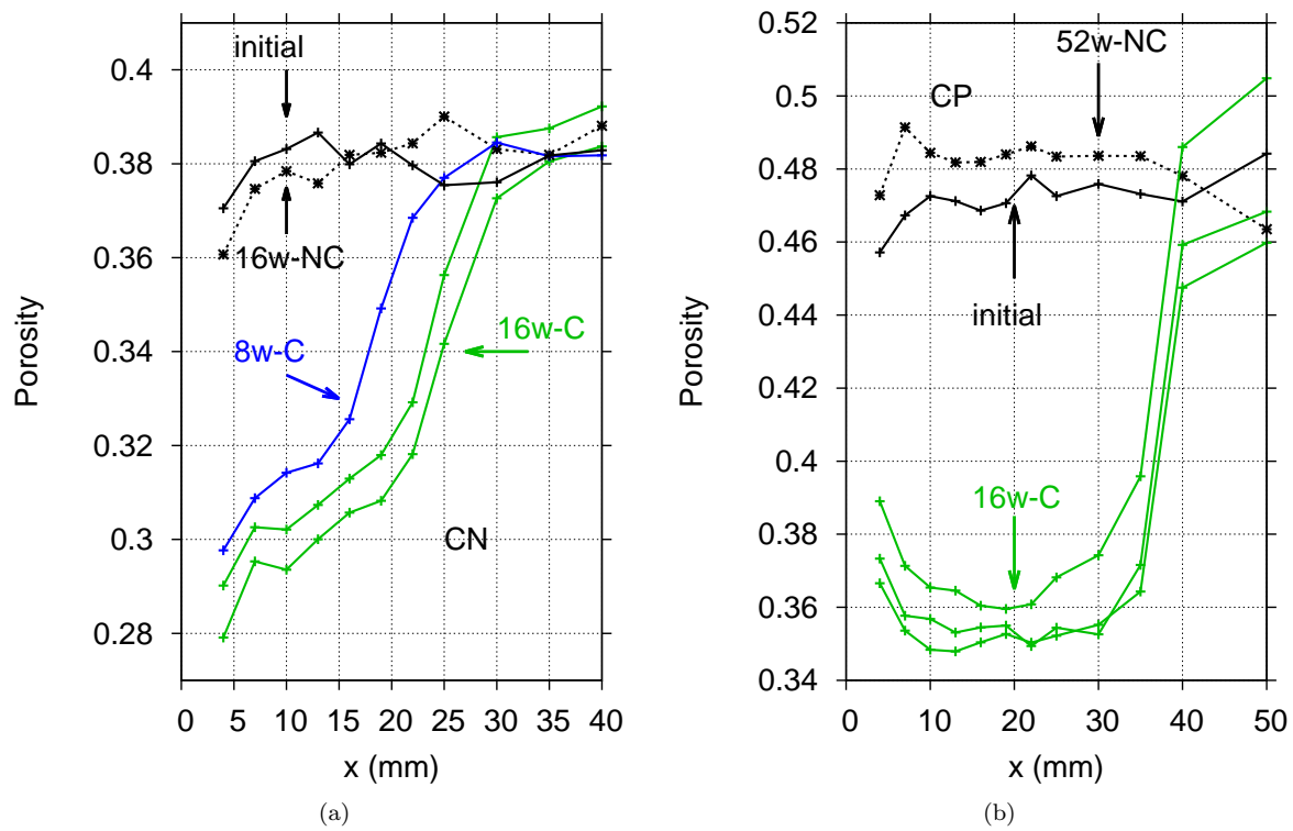
Figure 19: Porosity profile for both CN (a) and CP (b) at the initial state, after 56 and 112 days of carbonation (56d-C and 112d-C, resp), and after 112 days of drying (112d-NC).
