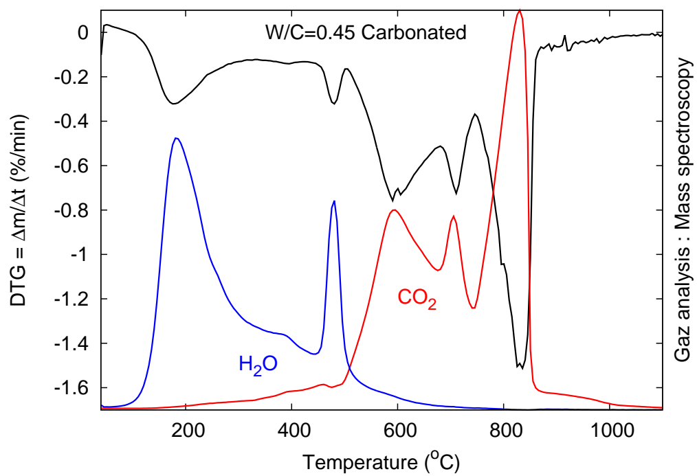
Figure 4: Mass spectrometry (MS) results for a highly carbonated sample of cement paste w/c = 0.45 . Comparison with the derivative of the mass loss during heating (DTG) peaks.
