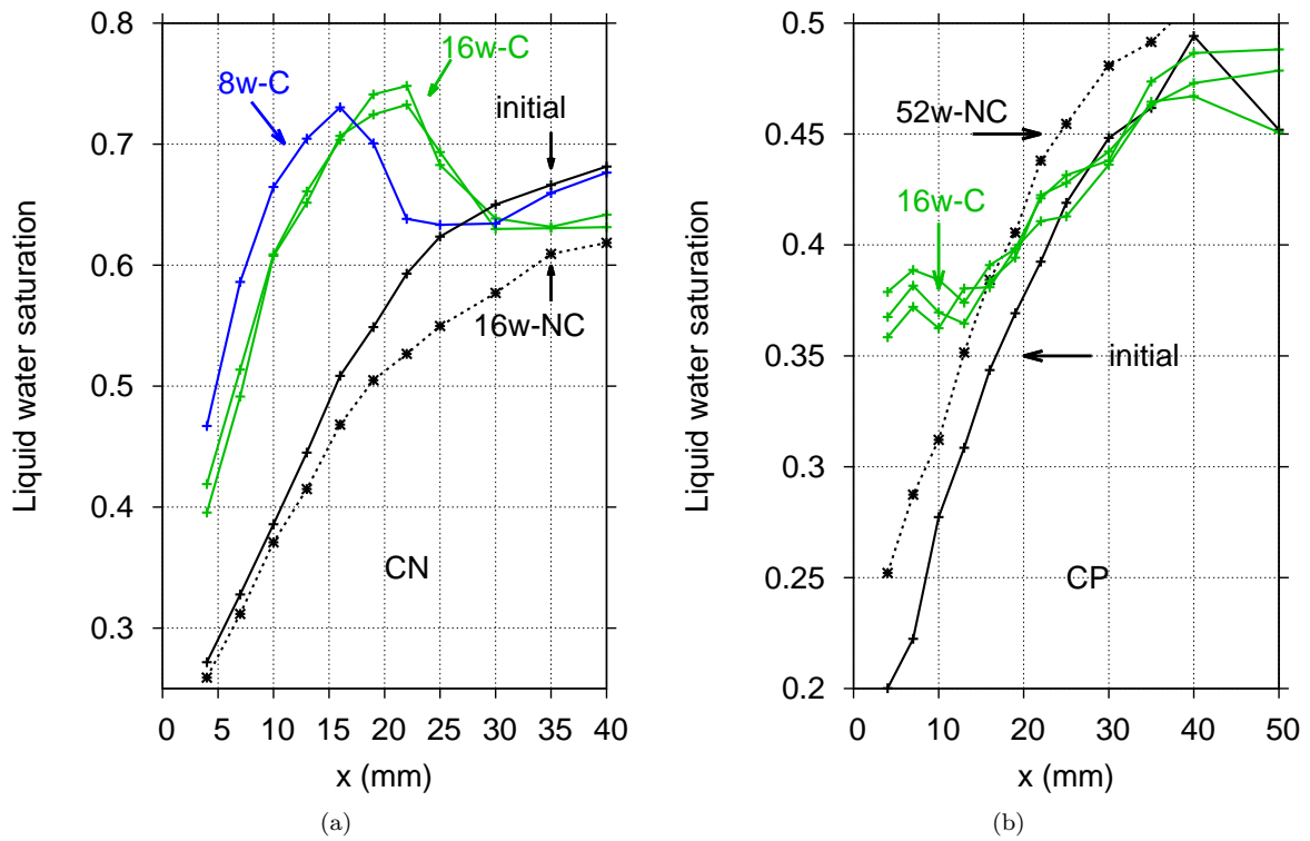
Figure 23: Water saturation profile obtained by GRAM for both CN and CP at the initial state, after 8 and 16 weeks of carbonation (8w-C and 16w-C, resp.). The profiles for the control specimens are illustrated (16 weeks for CN and 52 weeks for CP).
