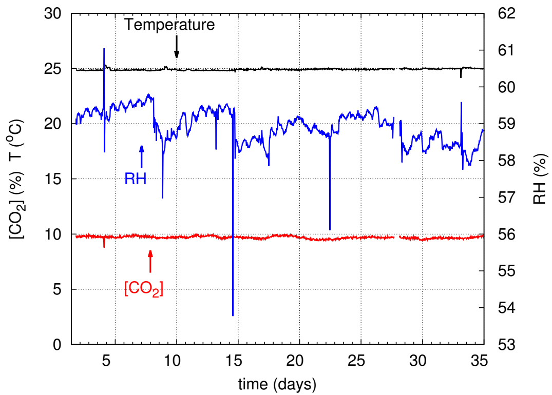
Figure 2: Monitoring example of the environmental parameters (monitoring window of 35 days).
