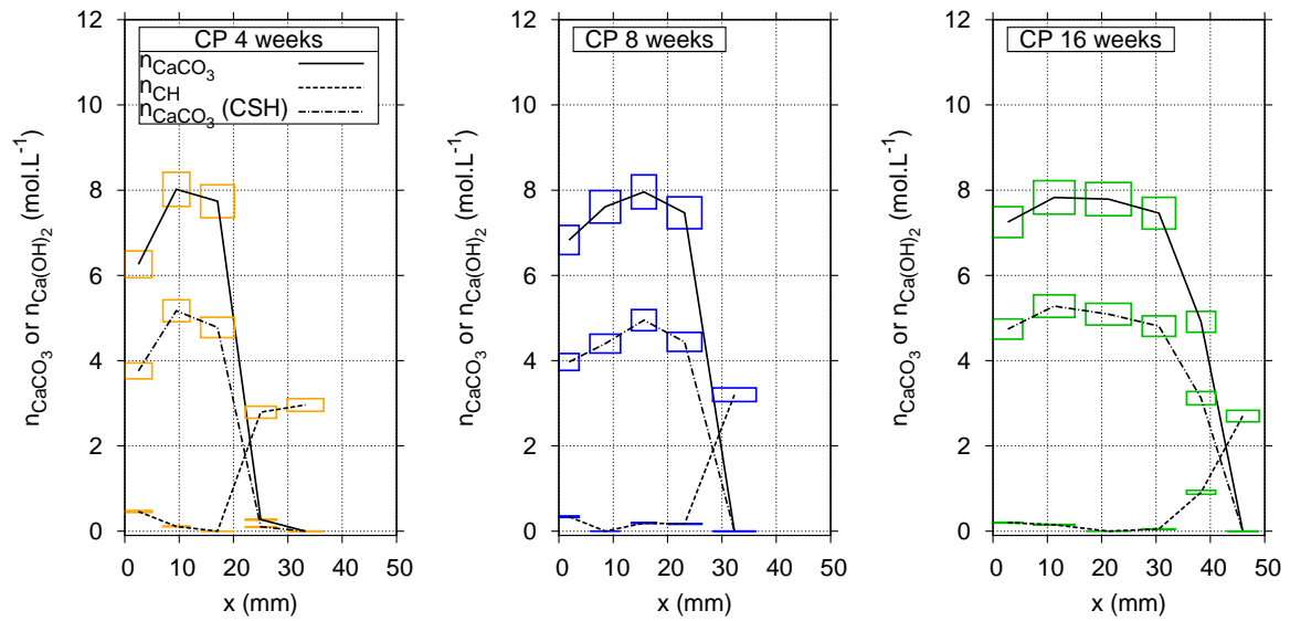
Figure 14: Carbonation profiles assessed by TGA-MS. Illustration of contents of CH and \bar{C}\bar{C} (for \bar{C}\bar{C} , total content and content only related to C-S-H carbonation are illustrated) after 4, 8 et 16 weeks of exposure to \text{CO}_2 . Case of CP paste.
