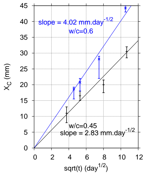
Figure 3: Carbonation depth determined by the phenolphthalein spray test on both CN ( w/c=0.45 ) and CP ( w/c=0.6 ) cement paste after 112 days of carbonation vs. square root of time.
