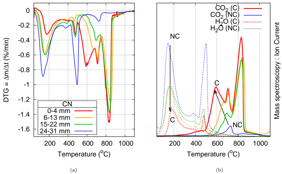
Figure 9: Diagrams of thermal analysis of samples sawn from the surface exposed to CO 2 to the core of a CN specimen exposed to 10% CO 2 during 8 weeks. (a) DTG diagrams and (b) mass spectroscopy diagrams.
