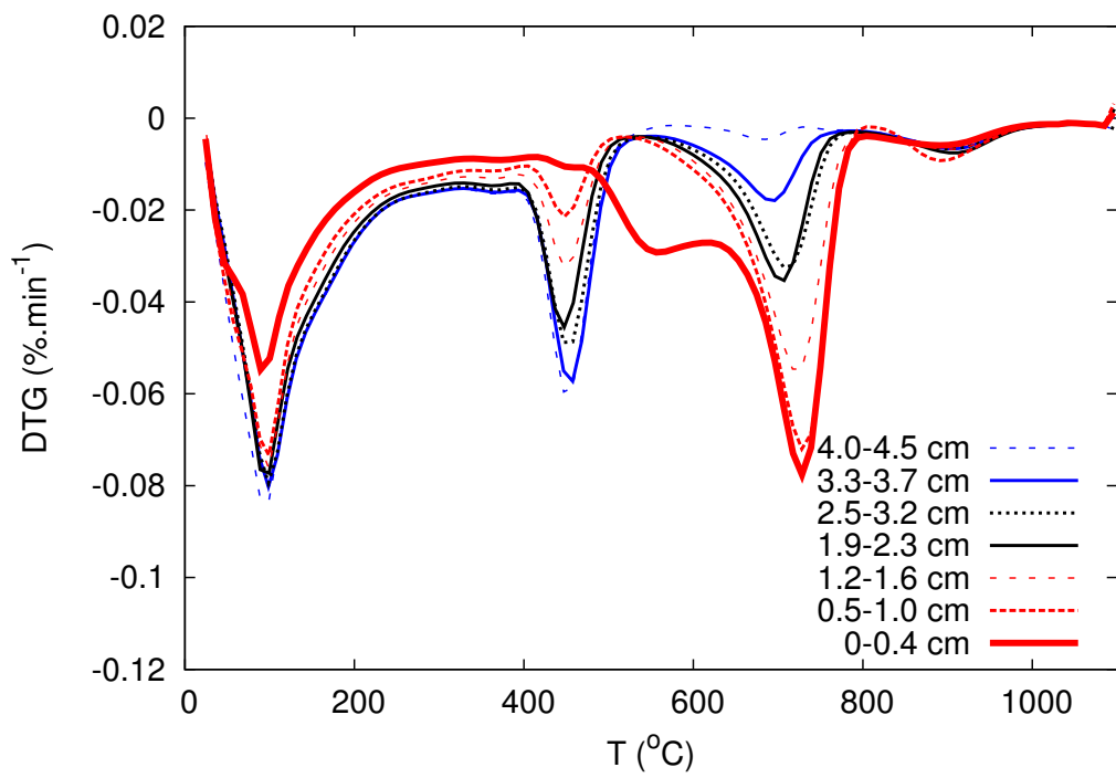
Figure 10: DTG diagrams of the slices sawn from the mortar specimen exposed to 10% CO 2 during 6 weeks.
