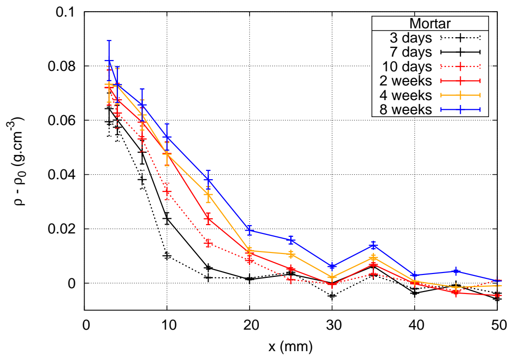
Figure 8: GRAM profiles for the mortar specimen ( w/c = 0.50 and s/c = 2 ).
