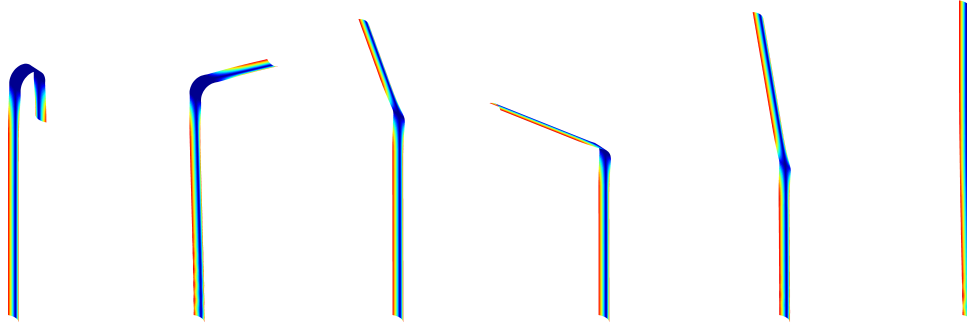
Figure 5: Deployment of a tape spring with a folded part.
