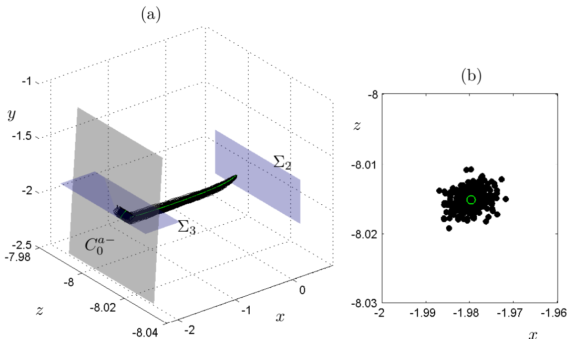
FIGURE 12. Computation of the transition map \Sigma_2 \rightarrow \Sigma_3 where the sections (blue) have been defined by the conditions x = 0.5 and y = -1.8 respectively. All paths have been started at (x, y, z) = (0.5, -2.1, -8) . There is one deterministic path (green) and 300 different realizations (black) for the stochastic case with M given by (7.7) and \sigma = 0.1 = \sigma' . The relevant part of the critical manifold C_0^{a+} (grey) is shown as well. (a) Phase space. (b) View of the landing points on the section \Sigma_3 where the landing point of the deterministic path is in the center of the green circle.
