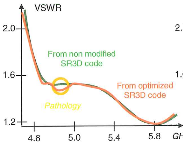
Figure 6 : Variations of the VSWR Interpolation code (red curve). Comparison with the reference (green curve). Level 0
