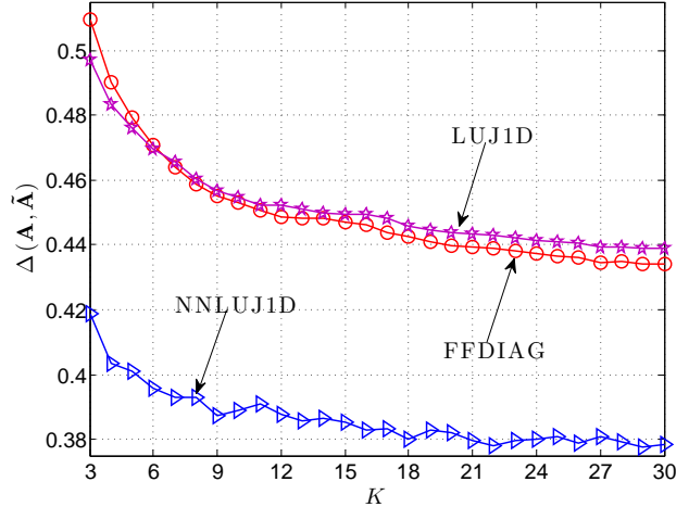
Fig. 2. The average error \Delta(\mathbf{A}, \tilde{\mathbf{A}}) evolution of compared algorithms versus the number of matrices K . The dimension of \mathbf{A} and the SNR are set to N=3 and \text{SNR}=5 dB, respectively.
