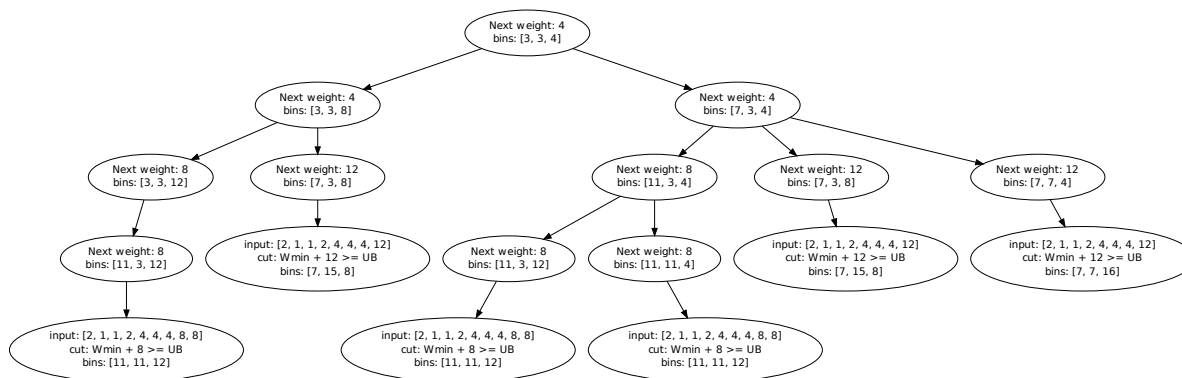
Figure A.7: Subtree 5, layout [3, 3, 4], items (2,1,1,2,4).
